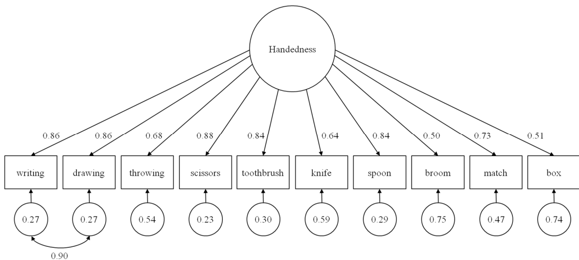
Figure 2. Confirmatory factor analysis of model 2. The digits close to the arrows refer to the standardized factor loadings. Error variances are represented in the circles at the bottom.
