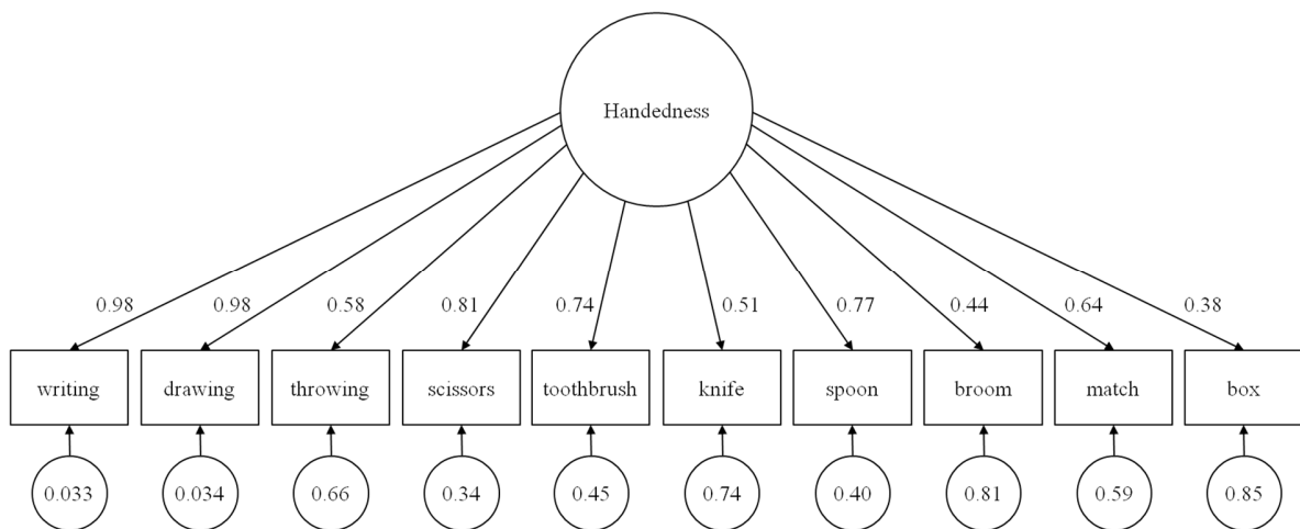
Figure 1. Confirmatory factor analysis of model 1. The digits close to the arrows refer to the standardized factor loadings. Error variances are represented in the circles at the bottom.
