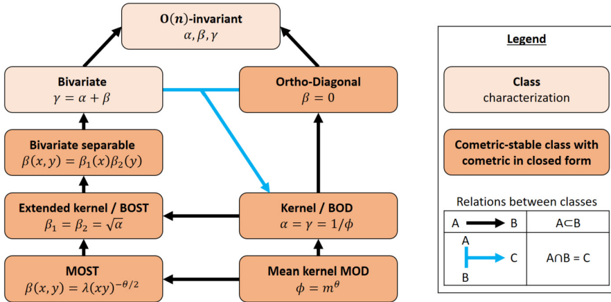
Fig. 1. Super-classes of kernel metrics.
