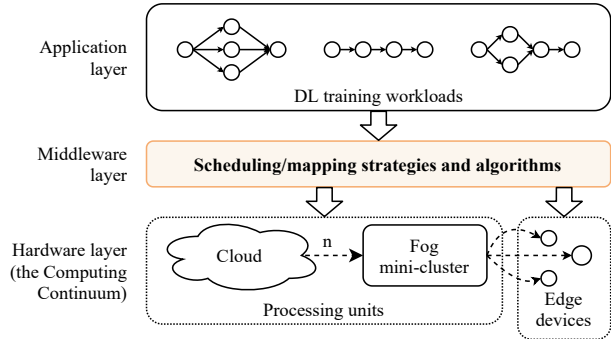
Fig. 1. Processing DL workloads on the Computing Continuum.
