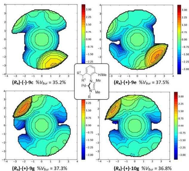
Figure 5. Steric contour maps of NHC ligands (complexes are oriented as shown in the central sketch).
