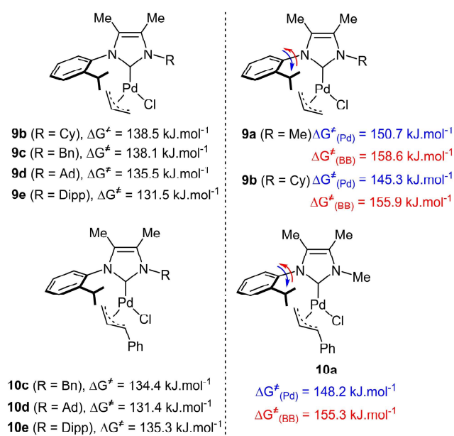
Figure 10. Values for the rotation barriers of Pd(NHC) complexes (left: experimentally determined; right DFT calculated).
