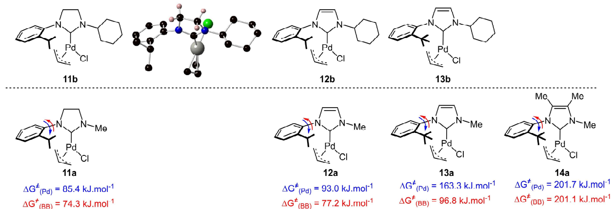
Figure 11. Influence of the backbone substitution on the rotation barriers.
