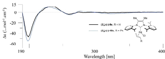
Figure 8. ECD spectra of first eluted complexes 9e and 10e .
