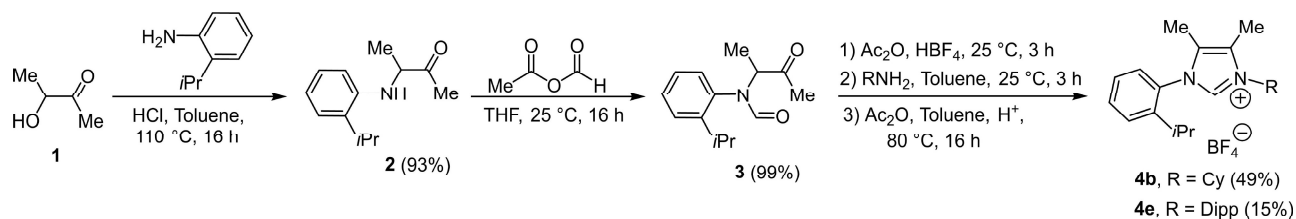
Scheme 1. Preparation of imidazolium salt 4 according to Fürstner's method. (Dipp = 2,6-diisopropylphenyl).
