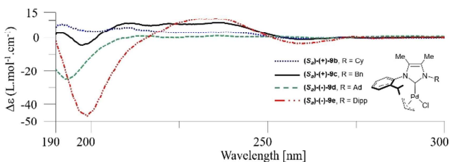
Figure 6. ECD spectra of first eluted complexes 9b–e .
