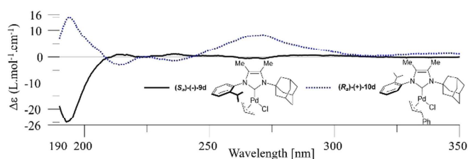
Figure 9. ECD spectra of first eluted complexes 9d and 10d .
