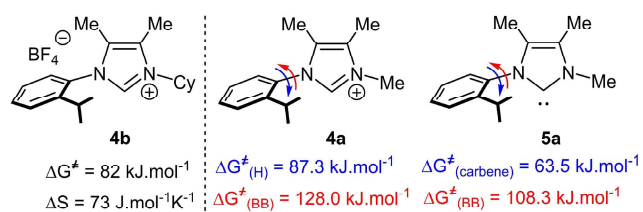
Figure 3. Values for the rotational barriers of imidazolium salts 4a and 4b and the corresponding free carbene 5a (left: experimentally determined; right DFT calculated).
