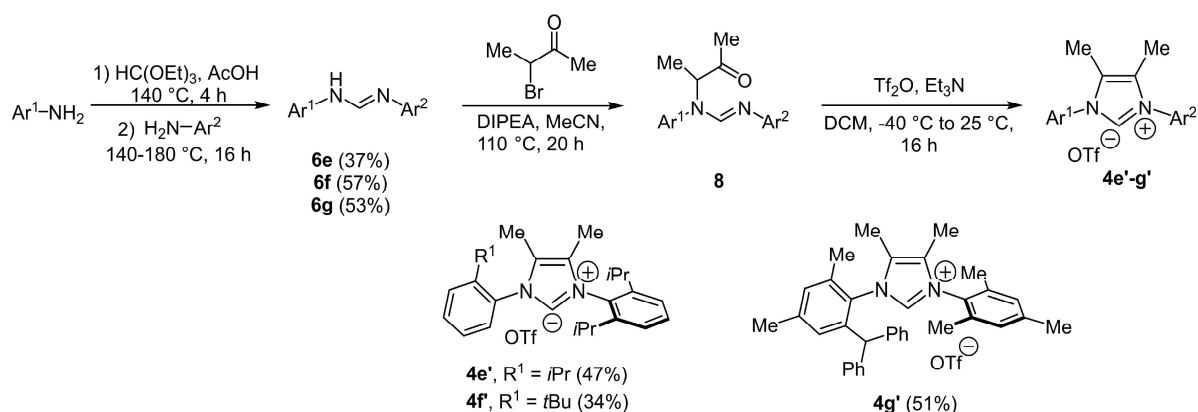
Scheme 3. Preparation of imidazolium salt 4 according to the procedure reported by Zhang and Shi.
