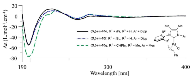
Figure 7. ECD spectra of first eluted complexes 10e–g .
