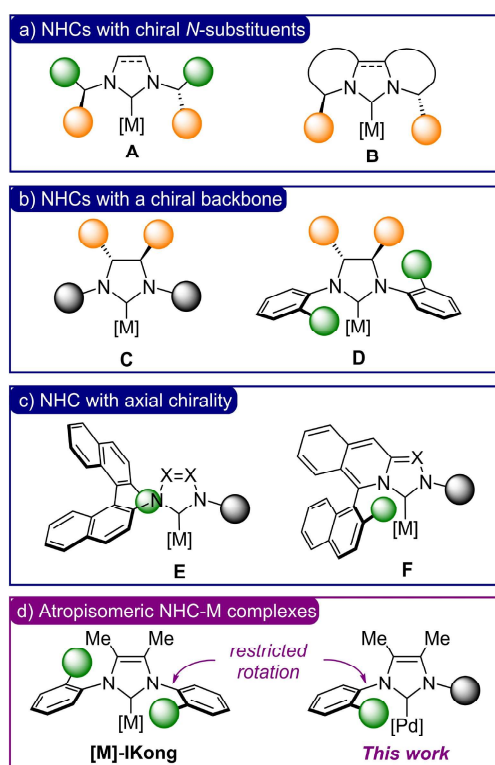
Figure 1. Designs of chiral monodentate NHC ligands.
