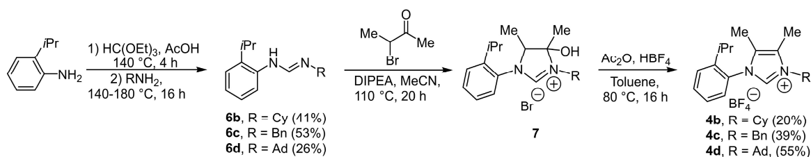
Scheme 2. Preparation of imidazolium salt 4 according to Glorius' synthetic procedure.
