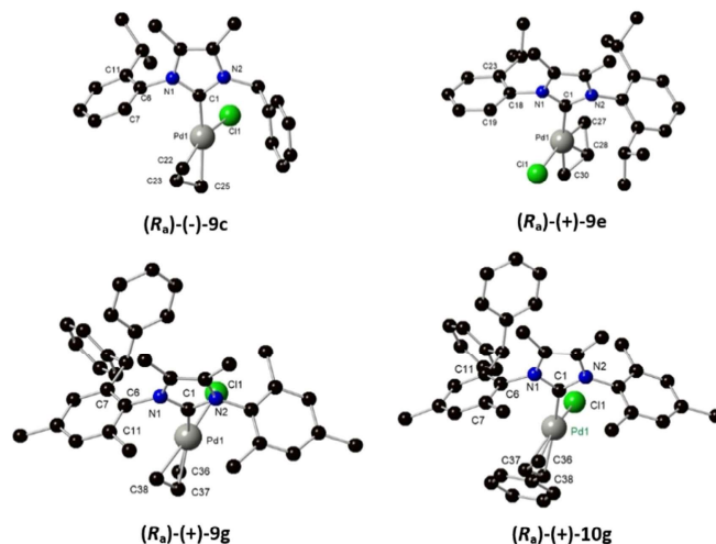
Figure 4. Ball-and-stick representations of enantiopure palladium complexes (hydrogens have been omitted for clarity).
