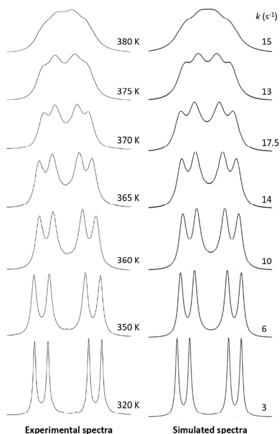
Figure 2. Variable temperature ^1\text{H} NMR spectra of imidazolium salt 4b in \text{C}_2\text{D}_2\text{Cl}_4 and the corresponding lineshape simulations.
