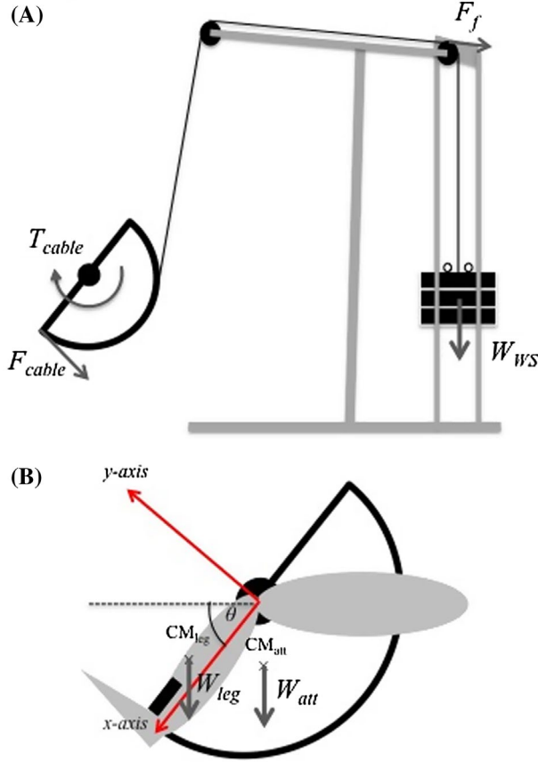
Figure 2. (A) Forces behind the resistive torque exerted by the cable ( T_{cable} ). For method A, T_{cable} was computed from the torque measured by the isokinetic dynamometer at a constant angular velocity and from the angular acceleration measured during the movement (Equation (4)). For method B, the force applied by the {cable + weight stack} system at the attachment point ( F_{cable} ) was multiplied by the radius of the half-circle metal component ( R = 0.395 m) (Equation (16)). F_{cable} was obtained from the friction force applied on the system, the weight of the weight stack and the linear acceleration of the weight stack (Equation (14)). (B) Cartesian coordinate system, where the origin, x -axis and y -axis correspond with the centre of knee joint, the axis defined by the {leg + resistance lever} system and a perpendicular axis forwardly oriented. The position of CM_{leg} , the leg centre of mass, was estimated from anthropometrical data and used to assess the torque due to W_{leg} , the weight of the lower leg. The position of CM_{att} , the attachment centre of mass, was estimated experimentally and used to determine the torque due to W_{att} , the weight of the attachment. (C) Preliminary study for friction force F_f assessment (adapted from Bosco et al., 1995). Weights were hanging on the opposite extremity of the cable ( W_H ) to lift the weight stack (WS). Weight stack motion was measured using an optoelectronic motion capture system and used to compute a_1 the linear acceleration of WS and W_H . Finally, F_f was computed from a_1 and a_2 , the linear acceleration of WS and W_H and W_1 and W_2 , the weight of WS and W_H .
