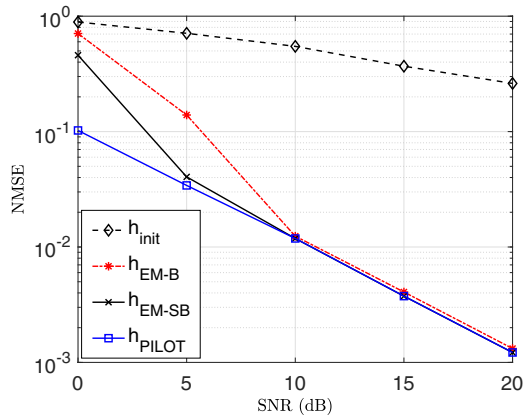
Figure 6: NMSE vs. SNR for blind ( h_{EM-B} ) and semi-blind ( h_{EM-SB} ) EM-based estimators benchmarked against the fully-pilot-based estimator ( h_{PILOT} ). We consider a quadratic model, 4-QAM modulation and a MIMO system with N_t = 2 , N_r = 4 , and M = 2 . h_{init} is included for reference and refers to a pilot-based estimator using available pilot symbols.
