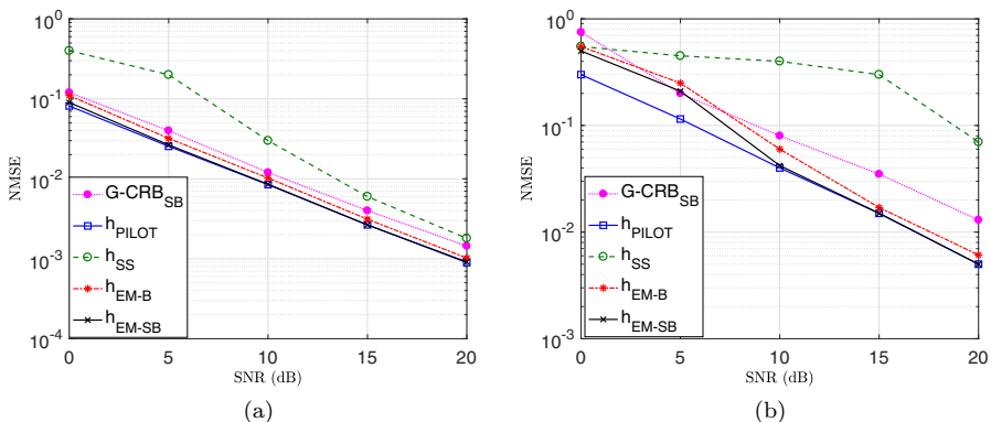
Figure 7: NMSE vs. SNR for subspace-based estimator ( h_{SS} ), blind ( h_{EM-B} ) and semi-blind ( h_{EM-SB} ) EM-based estimators benchmarked against the semi-blind Gaussian CRB ( G-CRBSB ) and the fully-pilot-based estimator ( h_{PILOT} ) (a) in the case of a quadratic model, 4-QAM modulation and N_r = 9 receive antennas (b) in the case of a cubic model and 16-QAM modulation.
