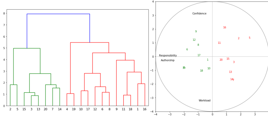
Fig. 2. Clustering of participants by metrics of operator's feelings about the chosen solution. (a) Hierarchical upward classification with k=2 groups. (b) Principal component analysis (axes 1 and 2).
