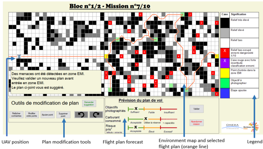
Fig. 1. HMI for preparing the mission of the intelligent agent.
