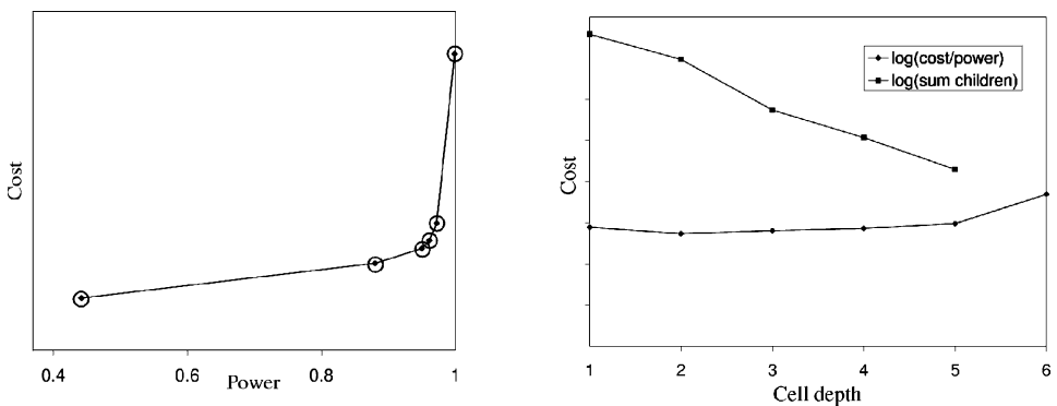
FIG. 10. Left: The pairs (\beta_l, c_l) for the fixed hierarchy used in the experiments. Right: top curve: l \rightarrow \log(C_l \times (c_{l+1}/\beta_{l+1})) where C_l is the number of children of a node at level l ; bottom curve: l \rightarrow \log(c_l/\beta_l) . The conditions of Corollary 1 are clearly satisfied.
