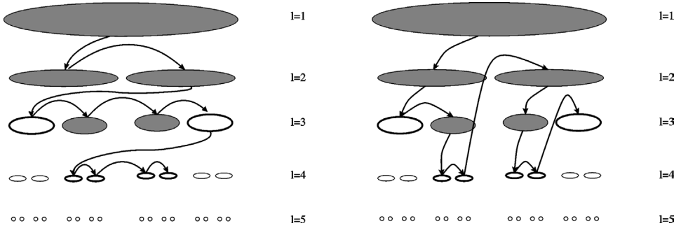
FIG. 3. Example of typical CTF strategies. Left: breadth-first ; right: depth-first .
