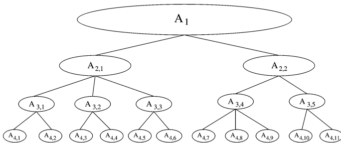
FIG. 1. Example of a (nonregular) tree-structured hierarchy of attributes.
