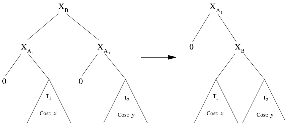
FIG. 4. The context of the switching property. Attribute A_1 is the coarsest attribute in the hierarchy; hence \Gamma(|B|) = b < \Gamma(|A_1|) = a .
