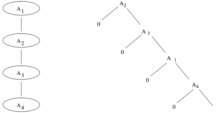
FIG. 2. Left: A vine-structured hierarchy of attributes for detecting one pattern. Right: An example of a vine-structured testing strategy for this hierarchy.
