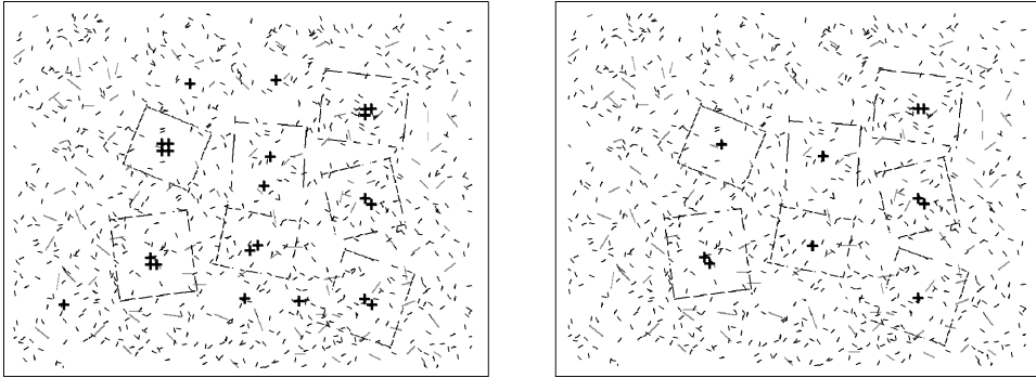
FIG. 11. Example of a detection result; the small crosses indicate the detected locations. Left: CTF detection only. Notice there are scattered false positives. Right: CTF search followed by template-matching. Nearly all the false positives are removed with virtually no increase in computation.
