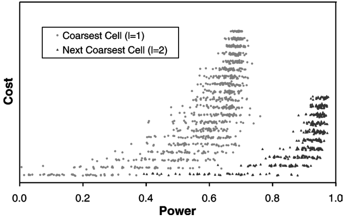
FIG. 8. Cost vs. power curve for attributes of depth one and two.
