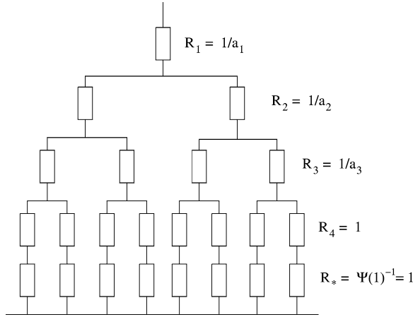
FIG. 5. Tree-structured resistor network identified with the attribute hierarchy, where a_l = \Gamma(|A_l|) is the complexity of attributes of level l and R_l = 1/a_l is the associated resistance; note that a_4 = 1 by convention for the bottom attributes. The last row of resistors represents the postprocessing stage. The conductance of this circuit is exactly the CTF testing cost of the attribute hierarchy when \Psi is the harmonic power function.
