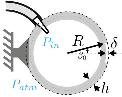
FIG. 1. Schematic of the clamped shell with an inlet for pressure control. The flexible tube connects at its other end to a vacuum tank so that when the line is open, P_{\text{in}} < P_{\text{atm}} (or P \equiv |P_{\text{in}} - P_{\text{atm}}| > 0 ). The relevant parameters are labeled: the nominal thickness h and midline radius R , imperfection depth \delta , and half-angular width of the imperfection \beta_0 .
