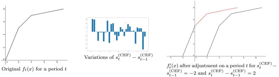
Figure 1: Updating the piecewise linear cost function f'_t
