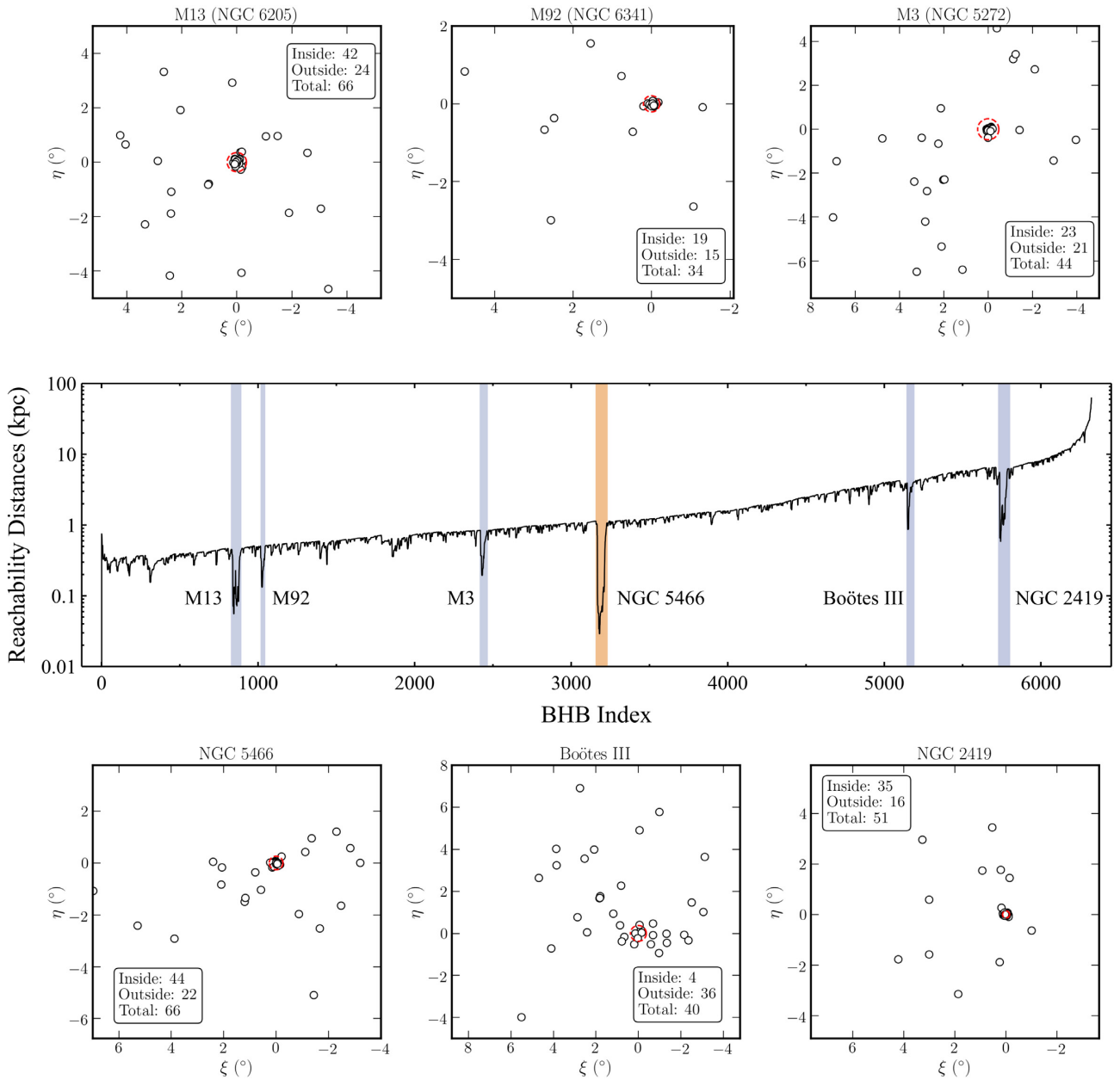
Figure 2. The dendrogram produced by OPTICS (central panel) with major substructures highlighted. The top and bottom rows show the tangent plane projection of the stars associated with each of these substructures, which correspond to known globular clusters or dwarf galaxies. For each, the red dashed circle corresponds to the literature measurement of the cluster’s tidal radius (or in the case of Boötes III, its half-light radius). Statistics for each object are listed describing the number of BHBs inside and outside r_t (or r_h ).
