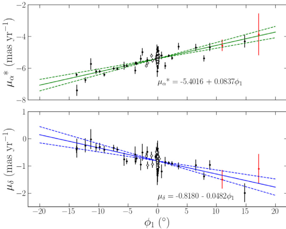
Figure 8. Proper motions, uncorrected for Solar reflex motion, as a function of \phi_1 . Point styles are the same as in Fig. 7 and additional members have been appended in red. The best-fitting trends are shown as solid lines. The dashed lines represent three times the standard error on the fitted slopes.
