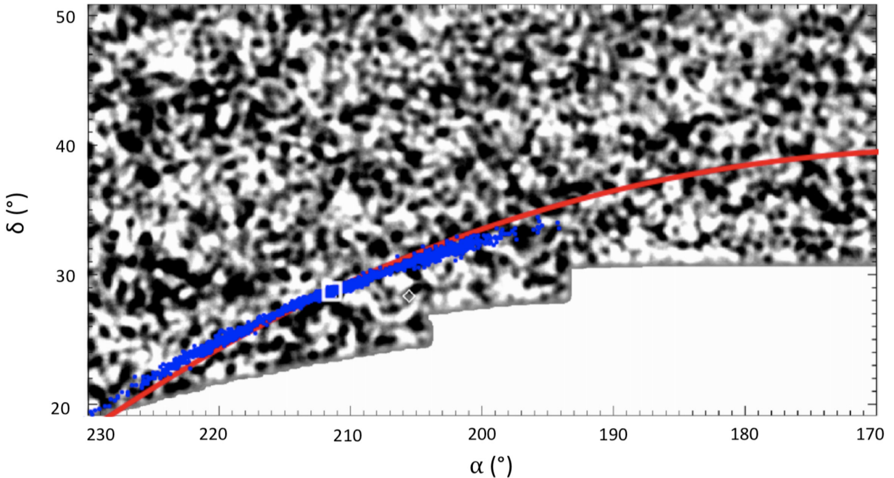
Figure 11. A direct comparison between the 45^\circ detection from Grillmair & Johnson (2006) to this work. The path of the extended tails is claimed to begin at (\alpha, \delta) = (230^\circ, 20^\circ) and end near (180^\circ, 42^\circ) . We overlay the great circle longitude ( \phi_1 ; red line) and GALA star particles (blue) on the matched filter map. Both diverge at approximately \alpha = 200^\circ compared to the original detection. NGC 5466 is represented with a white square and the nearby globular cluster M 3 (NGC 5272) as the diamond.
