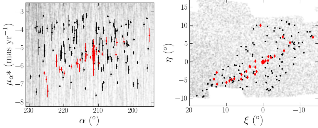
Figure 6. The left-hand panel shows the proper motions (not corrected for Solar reflex motion) of RGB stars as a function of \alpha , not corrected for Solar motion. The right-hand panel is the tangent plane of the same data. For both plots, the grey points are the full RGB sample, black are the filtered sample, and the red points represent stars surviving the sigma-clipping routine.
