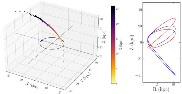
Figure 9. Orbit integrations of NGC 5466 in the Galactic frame. The left plot shows a 3D representation of the sprayed particles, where the scaled colours correspond to Galactocentric radius ( R ). We also show the Solar circle where the Sun is located at the blue point. In the right-hand panel, the blue and red trajectories are the backwards and forwards point-mass orbit integrations of NGC 5466.
