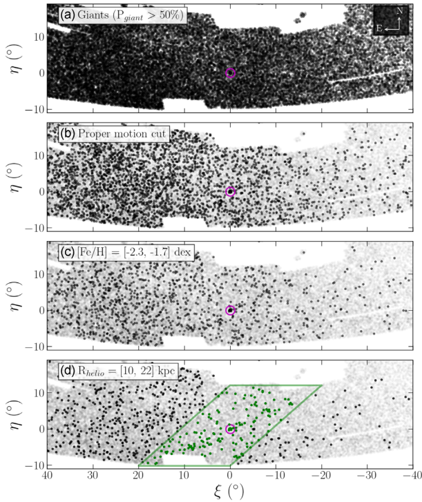
Figure 5. Tangent plane projection of giants in CFIS, centred on NGC 5466 (magenta circle). (a): Giants with P_{\text{giant}} > 50 per cent. (b): The grey points are the full sample as shown in (a), black points are the sample after filtering for proper motion. (c): Stars remaining after filtering for metallicity, [\text{Fe}/\text{H}] = [-2.3, -1.7] dex. (d): Stars remaining after filtering for distance, R_{\text{helio}} = [10, 22] kpc. Data within the green area are retained for further analysis.
