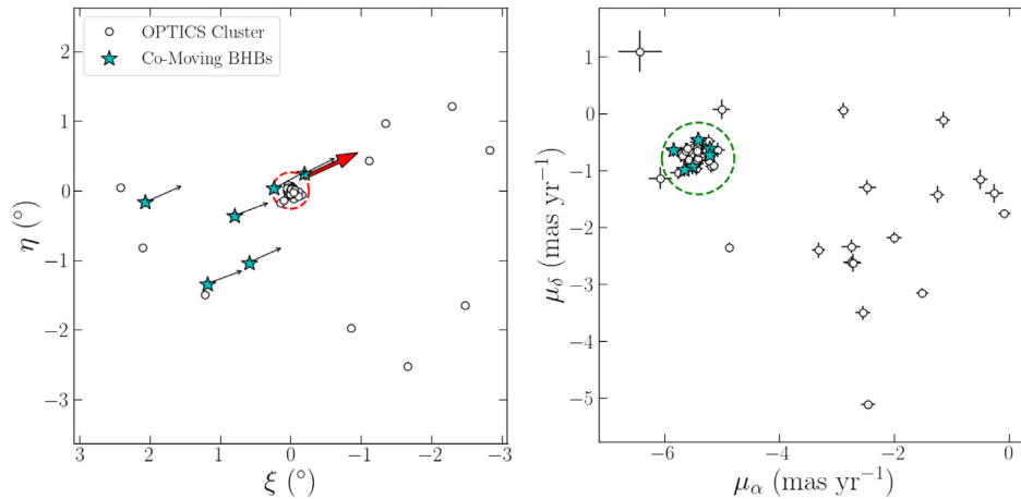
Figure 3. Left-hand panel: Tangent plane projection of the OPTICS BHBs identified as part of the NGC 5466 group (orange valley in Fig. 2). The red dashed circle corresponds to the tidal radius of the cluster, and the red arrow represents the proper motion of the cluster (Baumgardt et al. 2019) corrected for Solar reflex motion. Right-hand panel: Proper motion vector point diagram for the OPTICS BHBs of NGC 5466. The cluster of stars within the green circle correspond to stars moving with the same systemic proper motion as the cluster. We highlight the BHBs corresponding to stars moving with the cluster (outside r_t ) as cyan stars in both panels. Their (Solar reflex-corrected) proper motion vectors are also shown as black arrows in the tangent plane.
