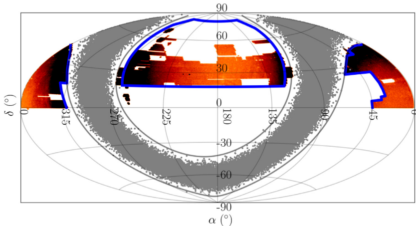
Figure 1. CFIS- u equatorial footprint. The blue outlines show the final CFIS area when the survey is complete ( \sim 5000 \text{ deg}^2 ), while the red/orange shaded regions are the fields available at the time of this study ( \sim 4000 \text{ deg}^2 ). The grey solid lines are located at b = \pm 20^\circ to highlight the boundary of CFIS in Galactic latitude; the grey points in this area highlight the approximate position of stars in the disc.
