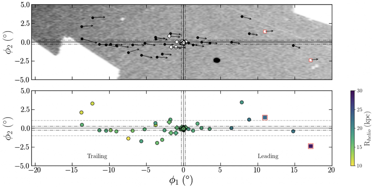
Figure 7. Gold sample RGBs (circles) and BHBs (diamonds) in the stream coordinate system. The vectors in the top panel are the proper motions corrected for Solar reflex motion, and rotated into the great circle frame. We show the limits of the CFIS footprint as the grey-filled region, where the dense circle at (\phi_1, \phi_2) \sim (5^\circ, -2.5^\circ) is the nearby cluster, M 3. Colours of stars in the bottom panel correspond to their heliocentric distances. Most of the stars identified are within 1^\circ of the \phi_2 plane, shown as the dashed lines in the bottom panel. The dash-dotted lines signify \pm r_t (tidal radius). The two additional member stars identified in Section 4.2 are plotted in red.
