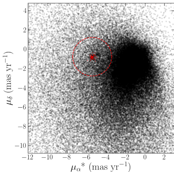
Figure 4. Vector point diagram of all giants ( P_{\text{giant}} > 50 per cent) in the CFIS data set. Stars within 1 - 2r_h of the cluster are shown as red points. The red dashed circle is the 2 \text{ mas yr}^{-1} boundary chosen to select stars with broadly similar proper motions to the globular cluster.
