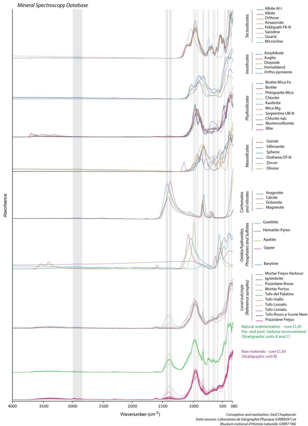
Figure 4: Overview of the mineral spectroscopy database showing: spectra of pure mineral classified by groups in comparison with the spectra from the current study including local reference outcrops, natural pre- and post-harbour sediments as well as raw construction material both obtained from core CL30. Grey lines are provided to improve the identification of absorbance peaks and to evidence spectra resemblance between the samples.
