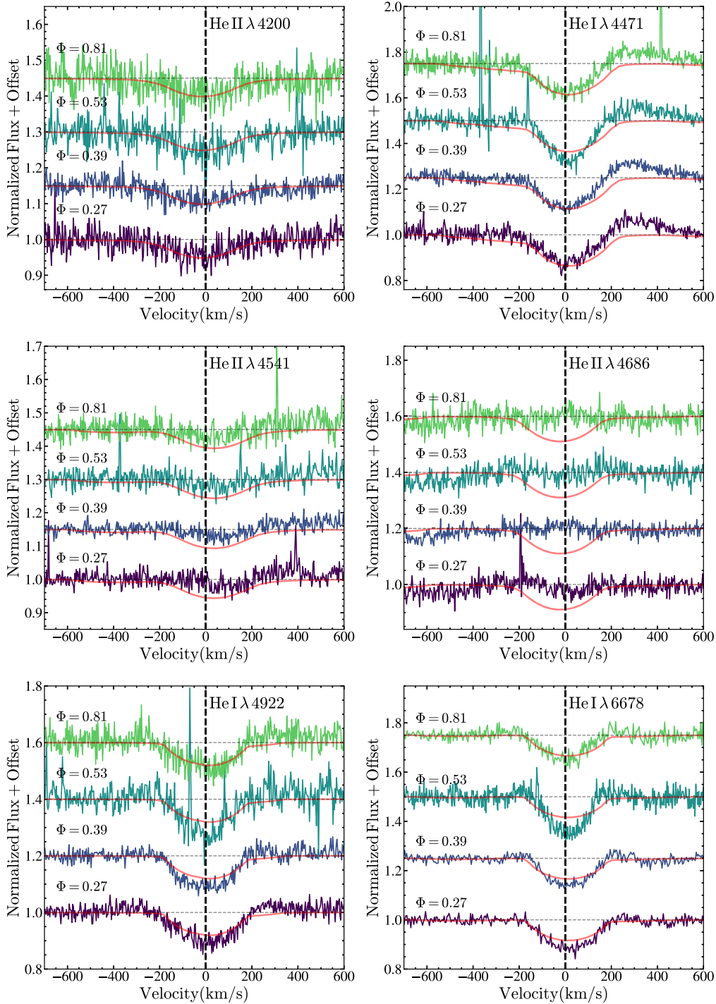
Figure 5. MIKE line profiles for He II \lambda 4200, He I \lambda 4471, He II \lambda 4541, He II \lambda 4686, He I \lambda 4922, and He I \lambda 6678. The TLUSTY BSTAR06 model atmosphere with T_{\text{eff}} = 30\,000 K and \log(g) = 3.25 is shown in red (Lanz & Hubeny 2003, 2007).
