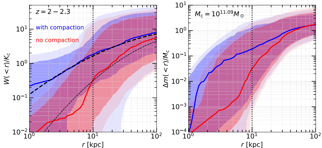
Figure 5. SatGen simulations of a cosmological sequence of satellites during one halo virial time at z \sim 2 , t_v \simeq 0.5 Gyr, corresponding to a redshift interval \Delta z \simeq 0.3 . Left: the energy deposited within radius r with respect to the kinetic energy in the 10 kpc cusp, W(<r)/K_c (left), with the dashed lines representing the fit used in Section 6 and listed in Table 1. Right: the satellite mass deposited inside r with respect to the host-cusp mass within 10 kpc, \Delta m(<r)/M_c . The host halo mass is M_v = 10^{12.5} M_\odot , with an NFW profile of c_{\text{NFW}} = 5 . The same for the steep-cusp profile is shown in Fig. G3 (supplementary material online). The fiducial run (blue) assumes compact satellites of m_v > 10^{11} M_\odot , while the reference run (red) assumes that all satellites are diffuse. Shown are the medians and the 68 per cent and 95 per cent percentiles over 600 random merger trees. The DZ profiles for the compact and diffuse satellites have the fiducial parameters (c, \alpha) = (7, 1) and (3, 0.5) , respectively. We see significant mass and energy deposit in the cusp for the compact satellites (valid for hosts of M_v > 10^{12} M_\odot at z > 1 ) and low mass and energy deposit for the case of diffuse satellites (approximating the situation in host haloes of M_v < 10^{11.5} M_\odot or at low redshifts).
