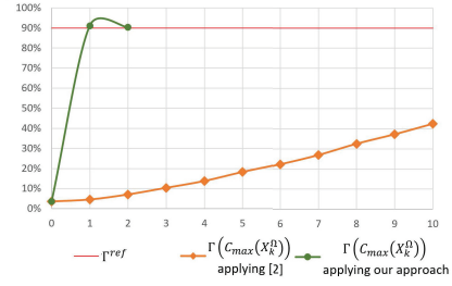
(b) Evolution of \Gamma(C_{\max}(X_k^{\Omega})) with the iterations
