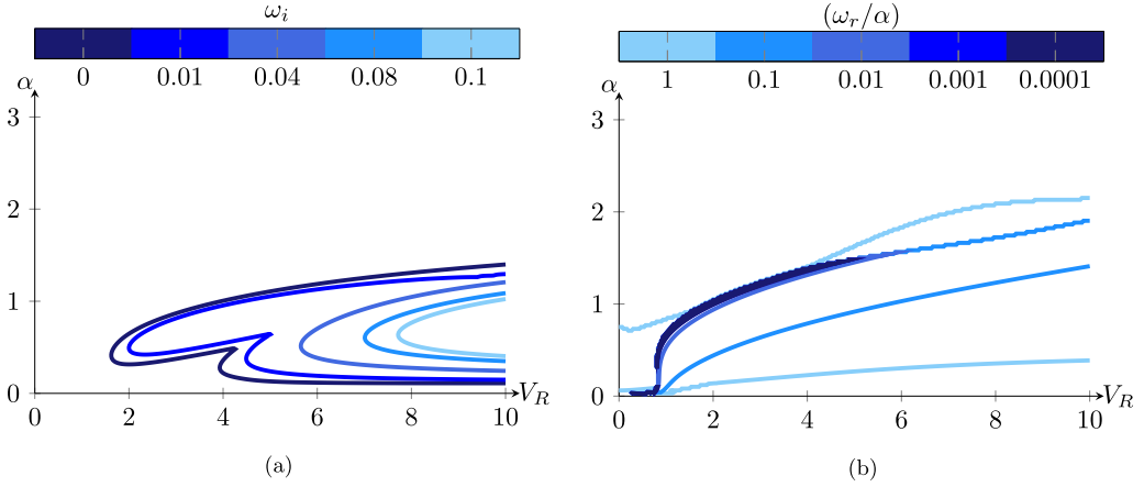
FIG. 5. Dispersion relation for leading varicose mode in (V_R, \alpha) plane for \text{Re} = 5000 , d_* = 10 , and B_* = 4 : contours of (a) growth rate \omega_i and (b) phase velocity \omega_r/\alpha .
