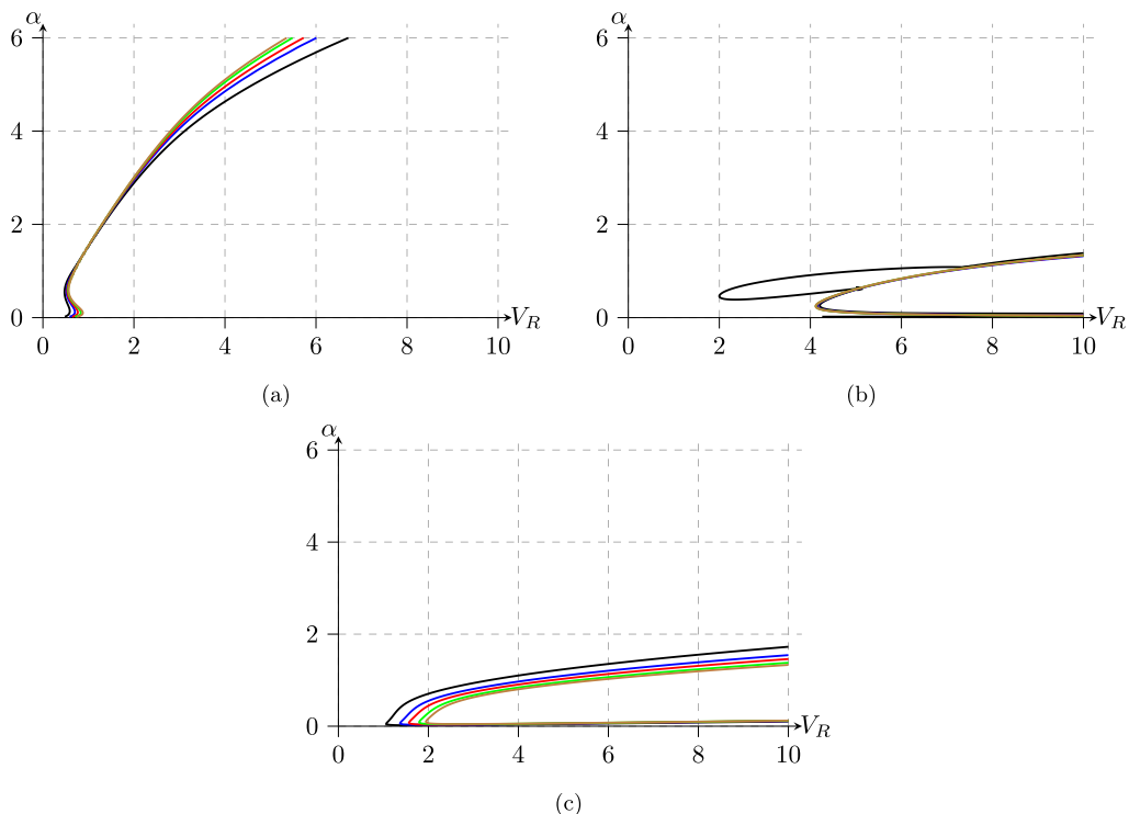
FIG. 7. Marginal curves for onset of varicose instability at B_* = 4 for \text{Re} = 10000, 40000, 80000, 160000, and 240000 (in black, blue, red, green, and brown respectively) and (a) d_* = 0 , (b) d_* = 10 , and (c) d_* = 100 .
