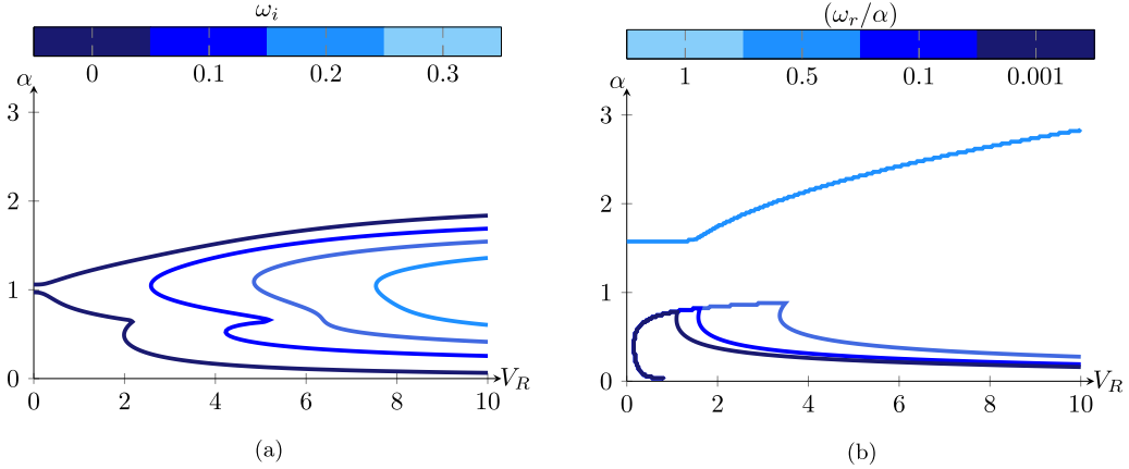
FIG. 8. Dispersion relation for leading sinuous mode in (V_R, \alpha) plane for \text{Re} = 8000 , d_* = 10 , and B_* = 4 : contours of (a) growth rate \omega_i and (b) phase velocity \omega_r/\alpha .
