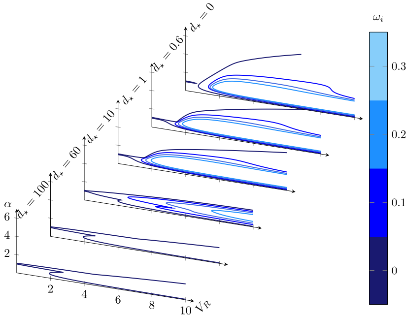
FIG. 9. Temporal growth rates \omega_i for the sinuous instability at \text{Re} = 8000 and B_* = 4 for d_* = 0, 0.6, 1, 10, 60 , and 100 . The contour levels are 0, 0.1, 0.2, and 0.3.
