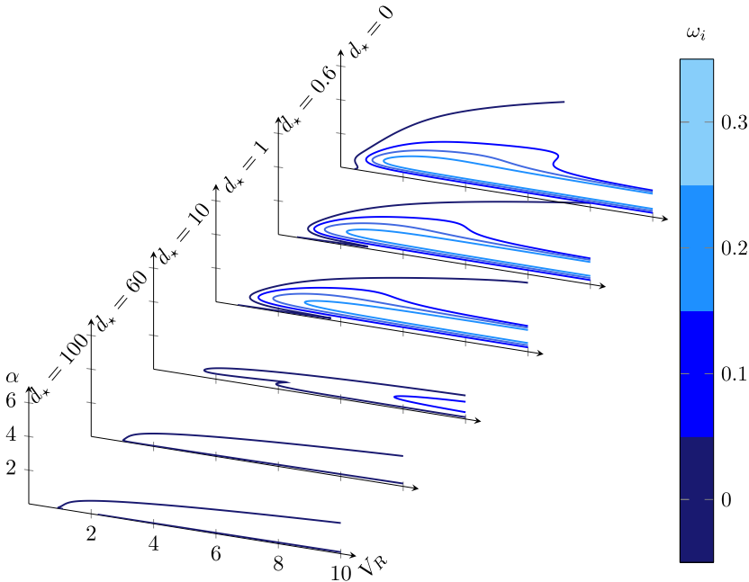
FIG. 6. Temporal growth rates \omega_i for the varicose instability at \text{Re} = 5000 and B_* = 4 for d_* = 0, 0.6, 1, 10, 60 , and 100 . The contour levels are 0, 0.1, 0.2, and 0.3.
