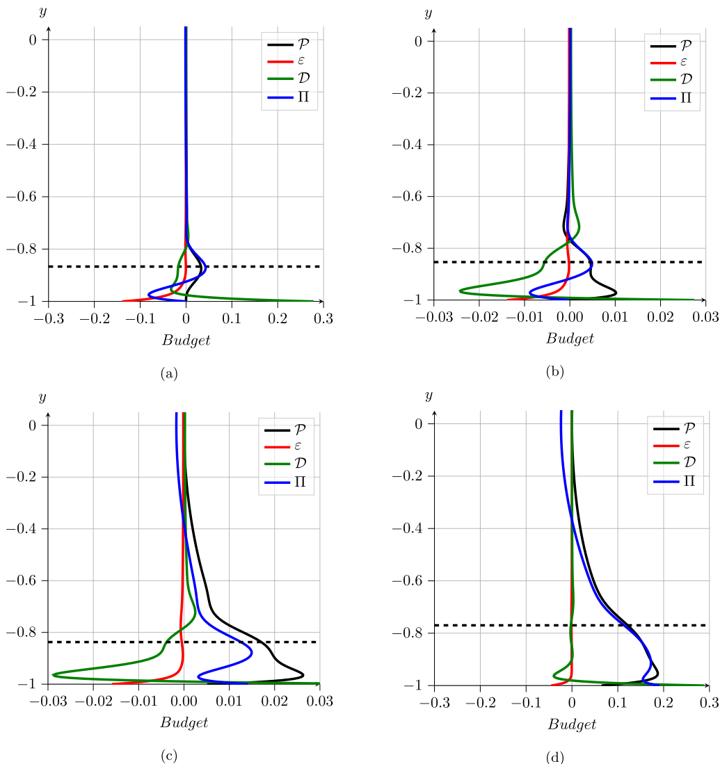
FIG. 18. Fluid kinetic energy budget profiles for most unstable TS mode at Re = 10000 , B_* = 1 , and (a) d_* = 0 , V_R = 0.03 , (b) d_* = 0 , V_R = 1 , (c) d_* = 0.14 , V_R = 1 , and (d) d_* = 0.2 , V_R = 1 . The wall-normal position of the critical layer is shown as a dashed line.
