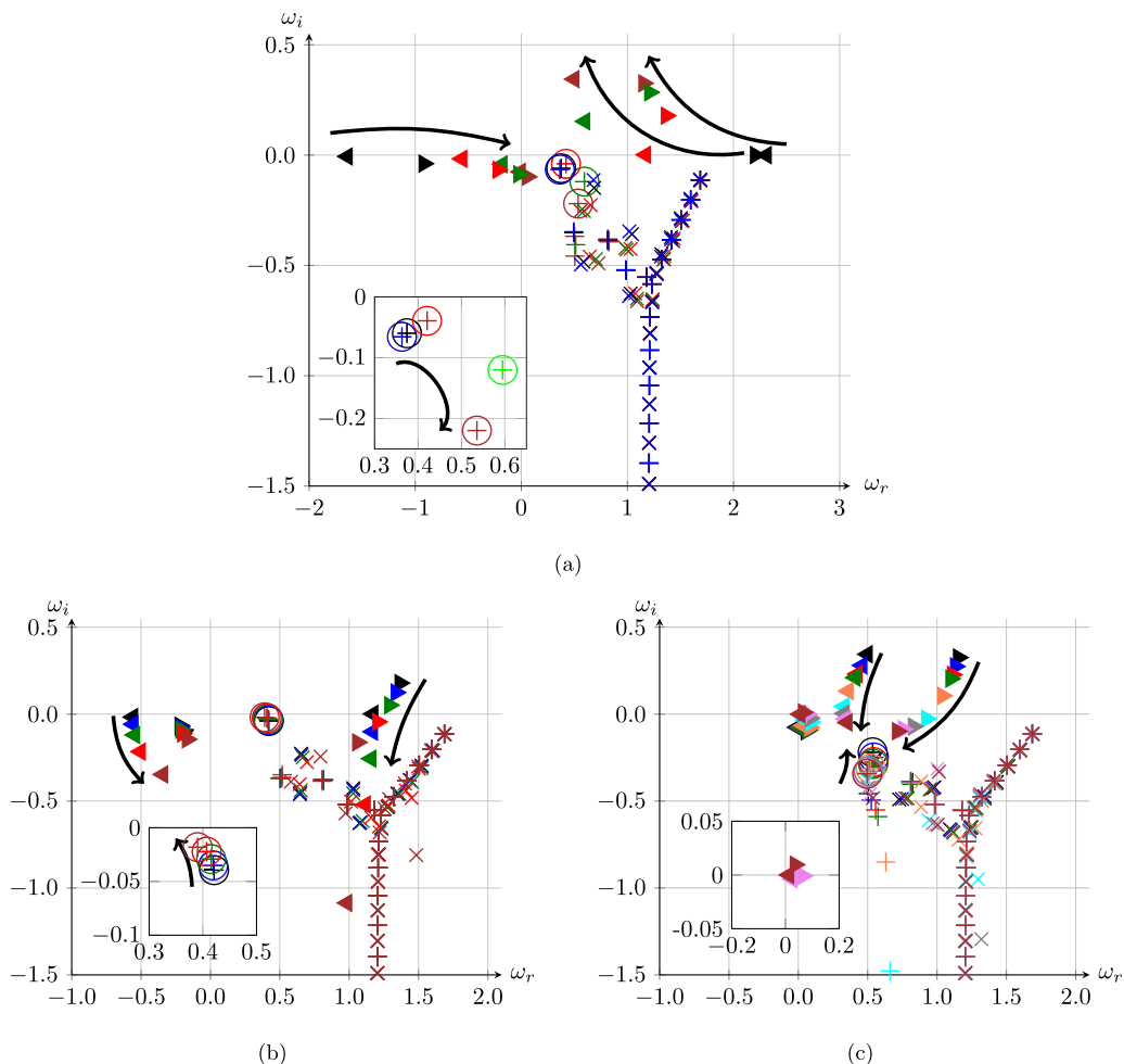
FIG. 3. Influence of V_R and d_* on eigenspectra for \alpha = 0.6 at \text{Re} = 7000 and B_* = 4 . (a) V_R = 0.01, 0.5, 1, 1.5, and 2 (in blue, black, red, green, and brown, respectively) at d_* = 0 . (b) d_* = 0, 0.2, 0.5, 1, and 2 (in black, blue, green, red, and brown, respectively) at V_R = 1 . (c) d_* = 0, 0.4, 0.8, 1, 2, 4, 6, 10, and 20 (in black, blue, red, green, orange, light blue, grey, pink, and brown, respectively) at V_R = 2 . Some mode trajectories are also represented.
