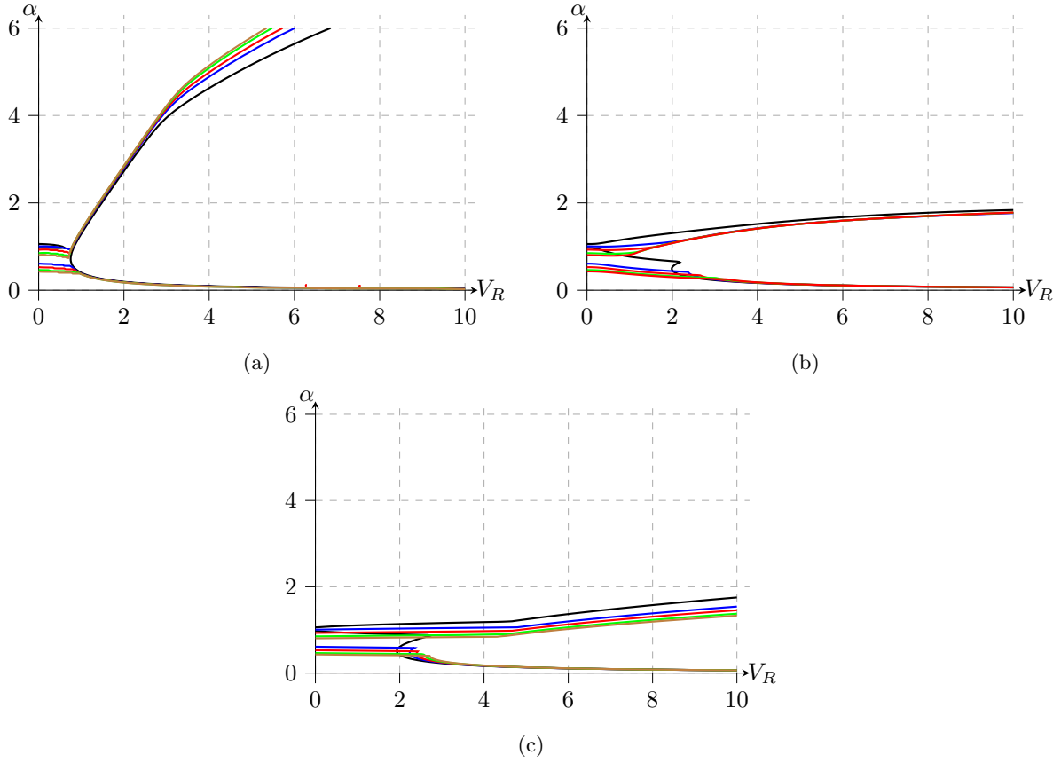
FIG. 10: Marginal curves for onset of sinuous instability at B_\star = 4 for Re = 10000 , 40000 , 80000 , 160000 and 240000 (in black, blue, red, green and brown respectively) and (a) d_\star = 0 , (b) d_\star = 10 and (c) d_\star = 100 .
