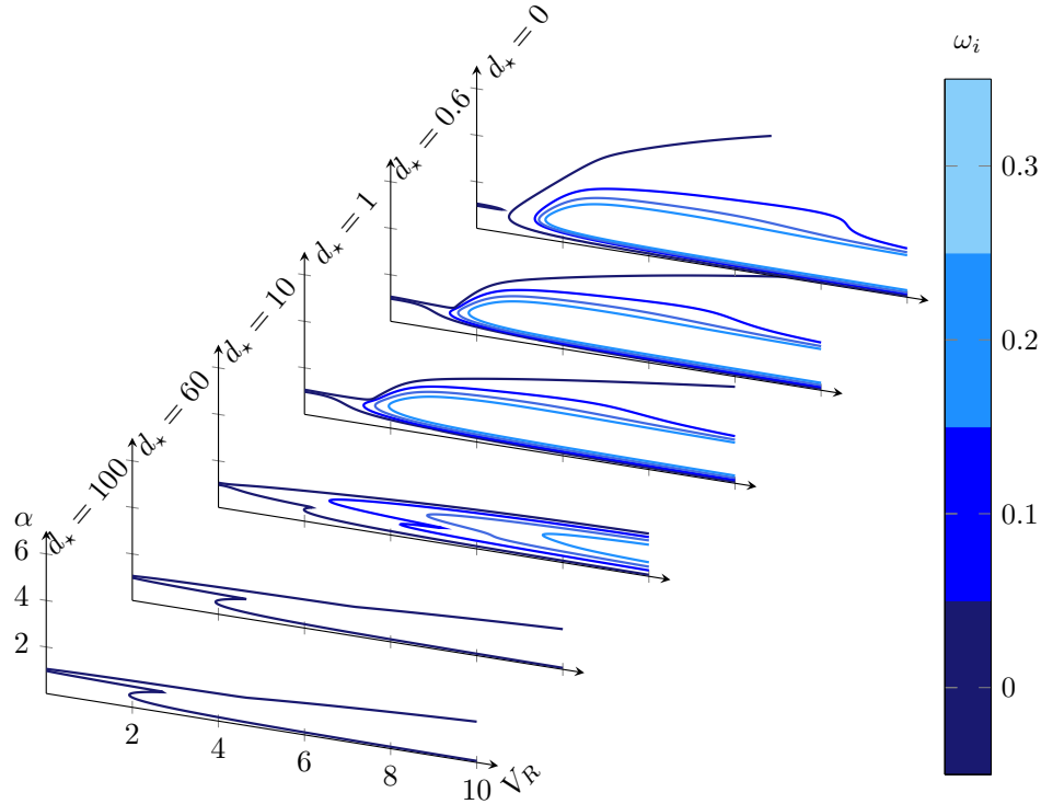
FIG. 9: Temporal growth rates \omega_i for the sinuous instability at Re = 8000 and B_\star = 4 for d_\star = 0, 0.6, 1, 10, 60 and 100 . The contour levels are 0, 0.1, 0.2 and 0.3.
