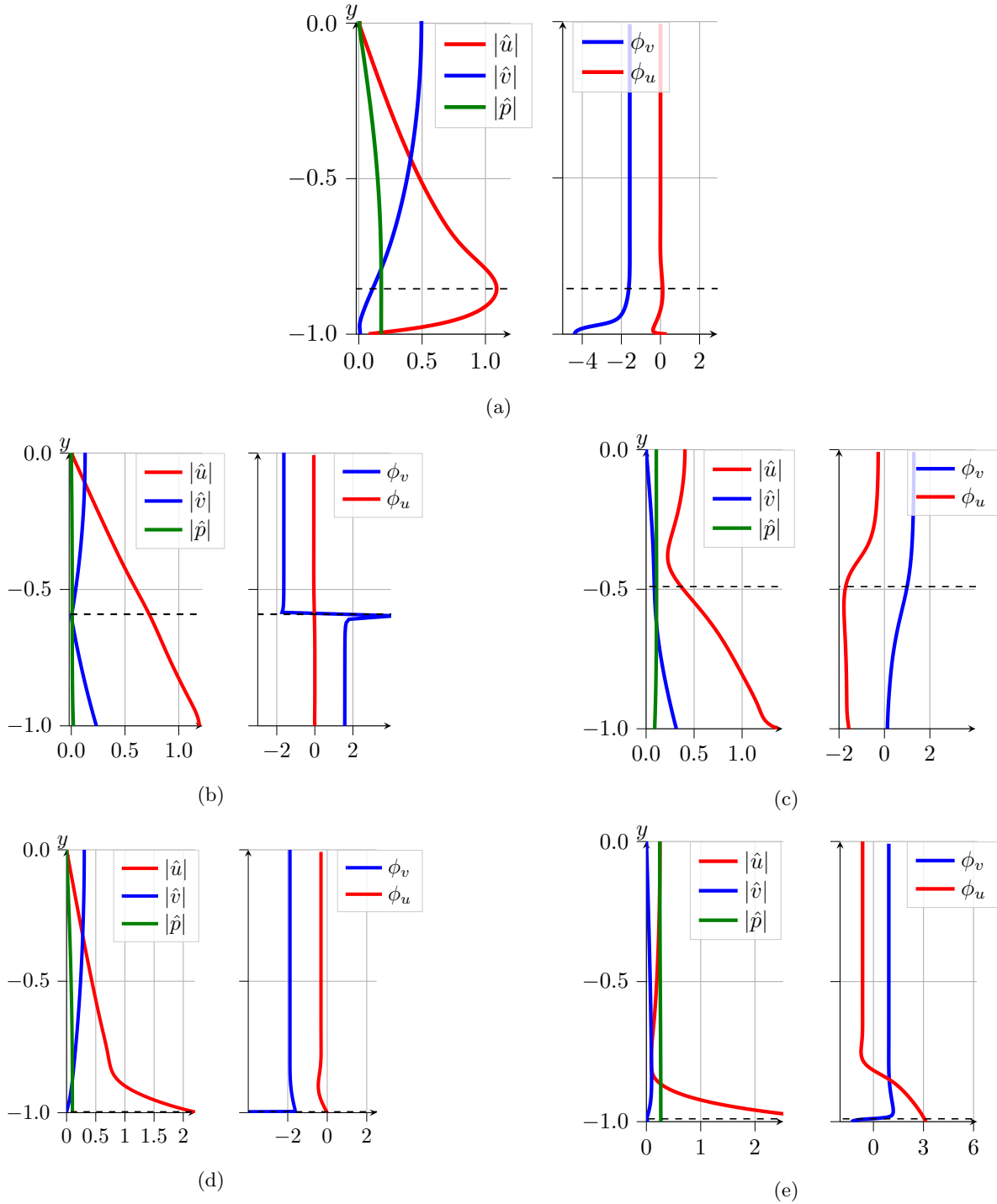
FIG. 4: Eigenfunctions for Re = 7000 and B_\star = 4 . (a) TS (sinuous) mode for \alpha = 1 , d_\star = 4 and V_R = 0.5 . (b) Sinuous TWF mode for \alpha = 0.6 , d_\star = 0 and V_R = 1 . (c) Varicose TWF mode for \alpha = 0.6 , d_\star = 0 and V_R = 1 . (d) Sinuous DIV mode for \alpha = 0.6 , d_\star = 20 and V_R = 2 . (e) Varicose DIV mode for \alpha = 0.6 , d_\star = 20 and V_R = 2 . The phase angles of eigenfunctions are denoted as \phi_u and \phi_v for u' and v' , respectively. The eigenfunctions are normalized to unit kinetic energy norm.
