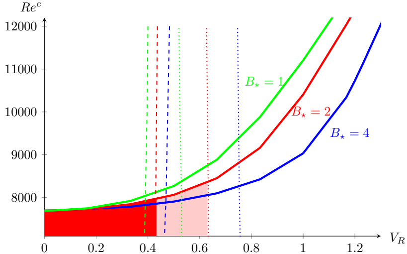
FIG. 15: The critical Reynolds number associated with TS instability is plotted as a function of V_R for B_\star = 1, 2 and 4 in full lines. Nearly vertical lines indicate onset of TWF instability for perturbations of sinuous (dotted lines) and varicose (dashed lines) symmetry. The colored regions correspond to stable configurations at B_\star = 2 , allowing only sinuous perturbations (light red) or all types of perturbations (solid red).
