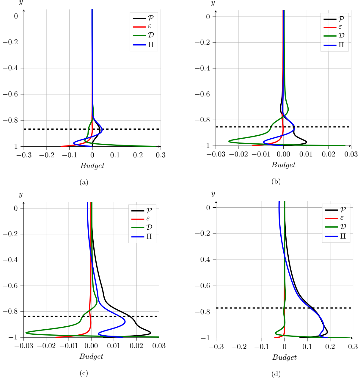
FIG. 18: Fluid kinetic energy budget profiles for most unstable TS mode at Re = 10000 , B_\star = 1 and (a) d_\star = 0 , V_R = 0.03 , (b) d_\star = 0 , V_R = 1 , (c) d_\star = 0.14 , V_R = 1 and (d) d_\star = 0.2 , V_R = 1 .
