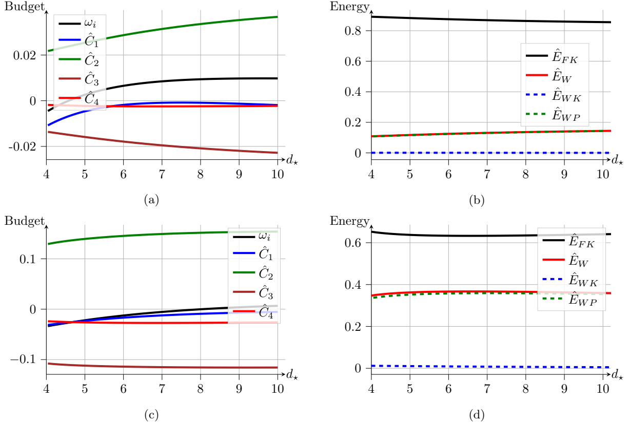
FIG. 20: Energy of most unstable DIV mode as d_* is increased at Re = 10000 , B_* = 1 and V_R = 2 . (a,c) Evolution of integrated total energy budget and (b,d) breakdown of total energy into its components for (a,b) sinuous and (c,d) varicose modes.
