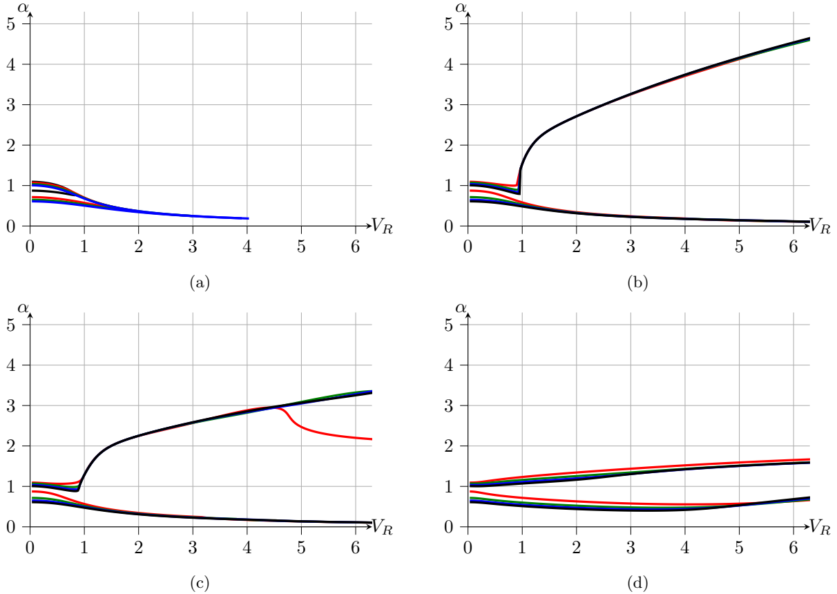
FIG. 12: Neutral curves for the TS mode for Re = 10000, 20000, 30000, 40000 (in black, red, green, blue, respectively) and B_* = 1 in the plane (\alpha, V_R) . (a) d_* = 0 , (b) d_* = 0.5 , (c) d_* = 1 and (d) d_* = 10 .
