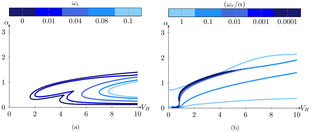
FIG. 5: Dispersion relation for leading varicose mode in (V_R, \alpha) -plane for Re = 5000 , d_\star = 10 and B_\star = 4 : (a) contours of growth rate \omega_i and (b) of phase velocity \omega_r/\alpha .
