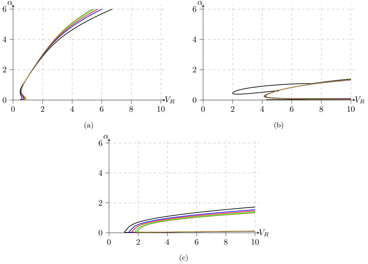
FIG. 7: Marginal curves for onset of varicose instability at B_* = 4 for Re = 10000 , 40000 , 80000 , 160000 and 240000 (in black, blue, red, green and brown respectively) and (a) d_* = 0 , (b) d_* = 10 and (c) d_* = 100 .
