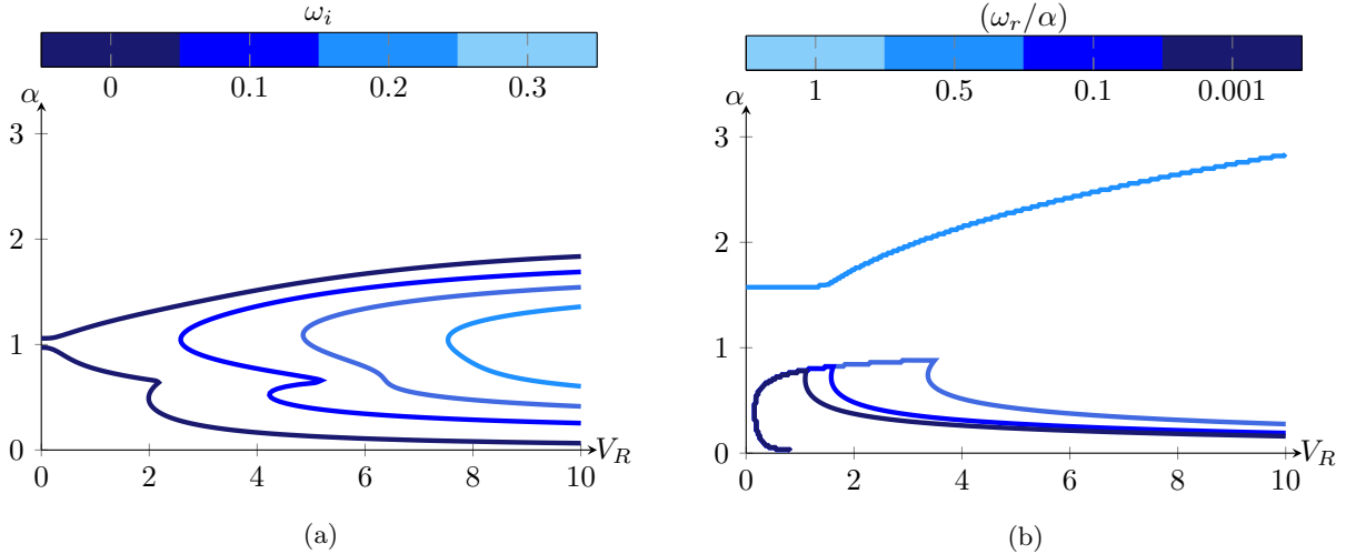
FIG. 8: Dispersion relation for leading sinuous mode in (V_R, \alpha) -plane for Re = 8000 , d_\star = 10 and B_\star = 4 : (a) contours of growth rate \omega_i and (b) of phase velocity \omega_r/\alpha .
