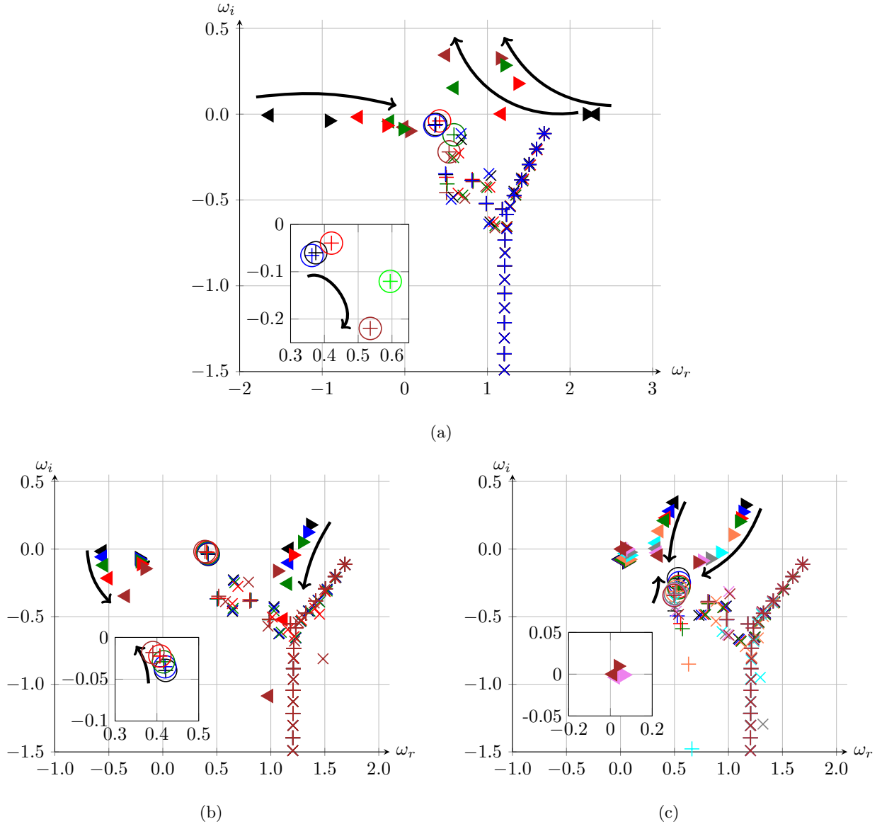
FIG. 3: Influence of V_R and d_* on eigenspectra for \alpha = 0.6 at Re = 7000 and B_* = 4 . (a) V_R = 0.01, 0.5, 1, 1.5 and 2 (in blue, black, red, green, and brown, respectively) at d_* = 0 . (b) d_* = 0, 0.2, 0.5, 1 and 2 (in black, blue, green, red and brown, respectively) at V_R = 1 . (c) d_* = 0, 0.4, 0.8, 1, 2, 4, 6, 10 and 20 (in black, blue, red, green, orange, light blue, grey, pink and brown, respectively) at V_R = 2 . Some mode trajectories are also represented.
