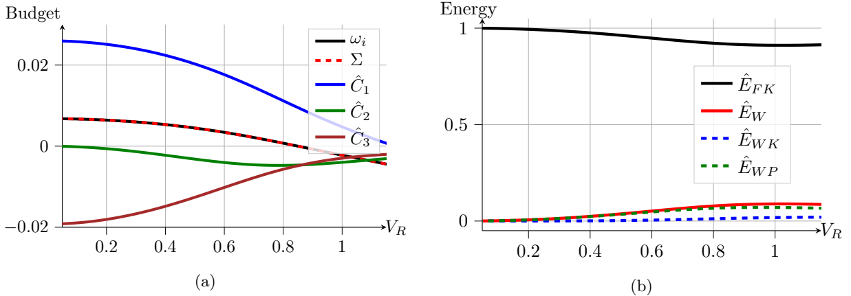
FIG. 17: Energy of most unstable TS mode as V_R is increased at Re = 10000 , B_* = 1 and d_* = 0 .
