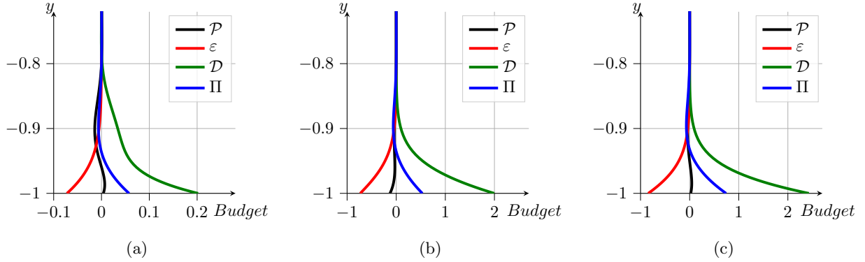
FIG. 21: Fluid kinetic energy budget profiles for most unstable DIV mode at Re = 10000 , B_* = 1 and V_R = 2 and (a) d_* = 5 sinuous mode, (b) d_* = 5 varicose mode, (c) d_* = 9 varicose mode.
