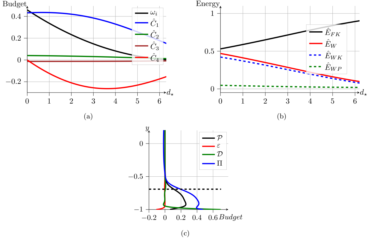
FIG. 23: Energy of most unstable varicose TWF mode as d_* is increased at Re = 10000 , B_* = 1 and V_R = 3 . (a) Evolution of integrated total energy budget. (b) Distribution of total energy as fluid and wall contributions. (c) Cross-channel profile of the fluid kinetic energy budget for d_* = 4 . The wall-normal position of the critical layer is shown in dashed-line.
