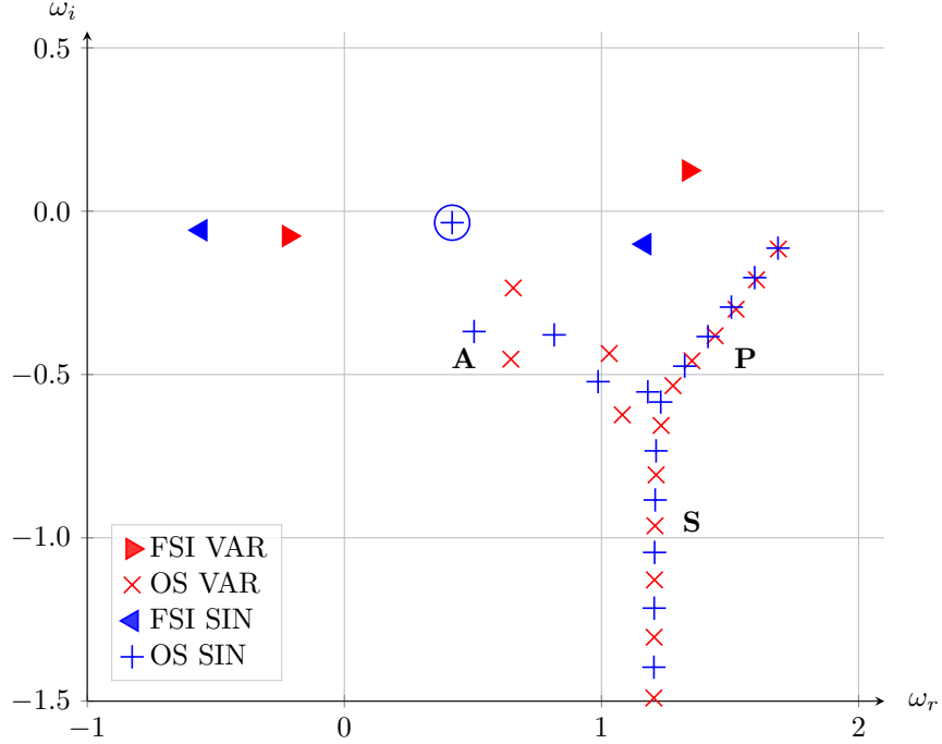
FIG. 2: Eigenvalue spectrum for perturbations with \alpha = 0.6 at Re = 7000 , V_R = 1 , B_\star = 4 and d_\star = 0.2 . Orr–Sommerfeld modes (+ sinuous and \times varicose) are located on three main branches (A, P and S) and dominated by TS mode (circle); four modes ( \triangleleft and \triangleright ) are due to fluid–structure interactions. Modes of varicose and sinuous symmetry are shown in red and blue respectively.
