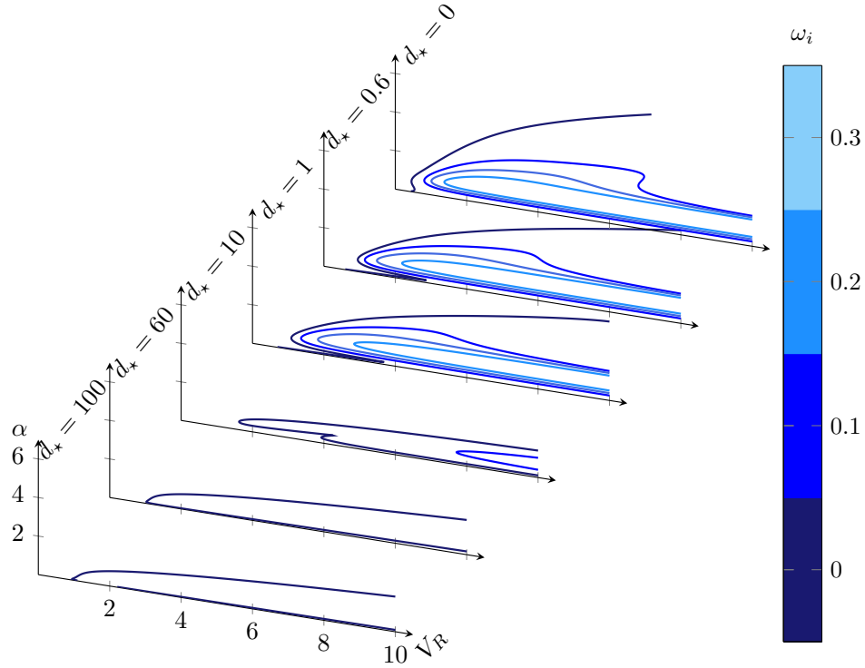
FIG. 6: Temporal growth rates \omega_i for the varicose instability at Re = 5000 and B_\star = 4 for d_\star = 0, 0.6, 1, 10, 60 and 100 . The contour levels are 0, 0.1, 0.2 and 0.3.
