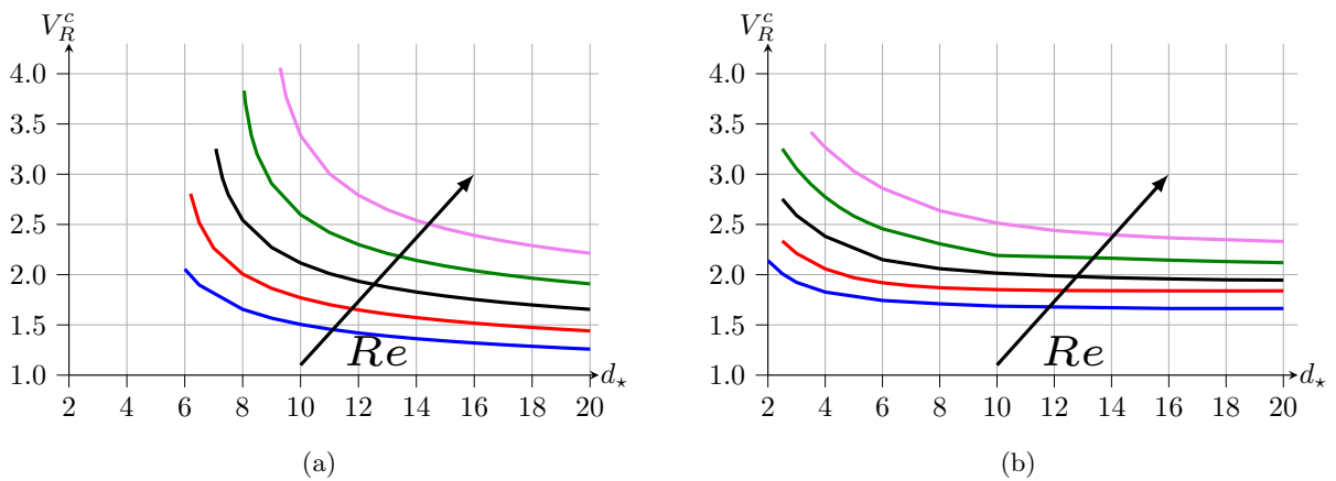
FIG. 13: Divergence mode. Critical reduced velocity distribution V_R^c with the wall damping parameter and for Re = 5000, 10000, 20000, 40000 and 80000 with B_* = 1 . (a) the varicose case, (b) the sinuous case.
