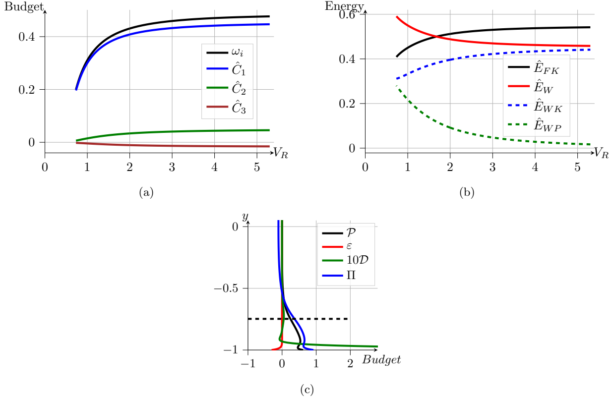
FIG. 22: Energy of most unstable varicose TWF mode as V_R is increased at Re = 10000 , B_\star = 1 and d_\star = 0 . (a) Evolution of integrated total energy budget. (b) Distribution of total energy as fluid and wall contributions. (c) Cross-channel profile of the fluid kinetic energy budget for V_R = 3 . The wall-normal position of the critical layer is shown in dashed line.
