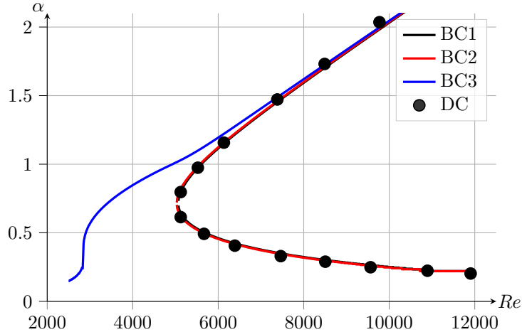
FIG. 24: Neutral curves. Sinuous configuration. Effects of the boundary conditions.
