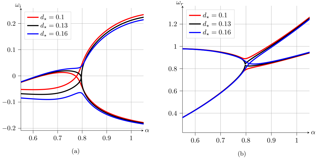
FIG. 11: Dispersion relation for the two leading sinuous modes at Re = 10000 , B_* = 1 and V_R = 1 . (a) empirical growth rate \omega_i and (b) frequency \omega_r . Branch switching occurs near \alpha = 0.8 and d_* = 0.13 .
