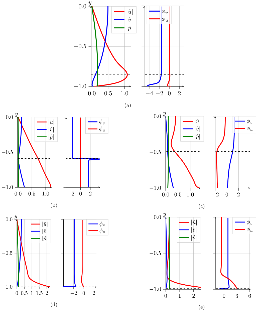
FIG. 4. Eigenfunctions for Re = 7000 and B_* = 4 . (a) TS (sinuous) mode for \alpha = 1 , d_* = 4 , and V_R = 0.5 . (b) Sinuous TWF mode for \alpha = 0.6 , d_* = 0 , and V_R = 1 . (c) Varicose TWF mode for \alpha = 0.6 , d_* = 0 , and V_R = 1 . (d) Sinuous divergence mode for \alpha = 0.6 , d_* = 20 , and V_R = 2 . (e) Varicose divergence mode for \alpha = 0.6 , d_* = 20 , and V_R = 2 . The phase angles of eigenfunctions are denoted as \phi_u and \phi_v for u' and v' , respectively. The eigenfunctions are normalized to the unit kinetic energy norm.
