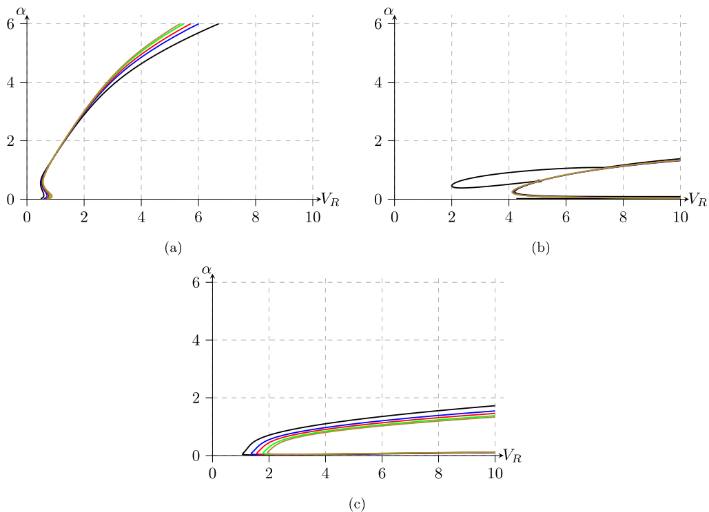
FIG. 7. Marginal curves for onset of varicose instability at B_\star = 4 for \text{Re} = 10000, 40000, 80000, 160000, and 240000 (in black, blue, red, green, and brown respectively) and (a) d_\star = 0 , (b) d_\star = 10 , and (c) d_\star = 100 .
