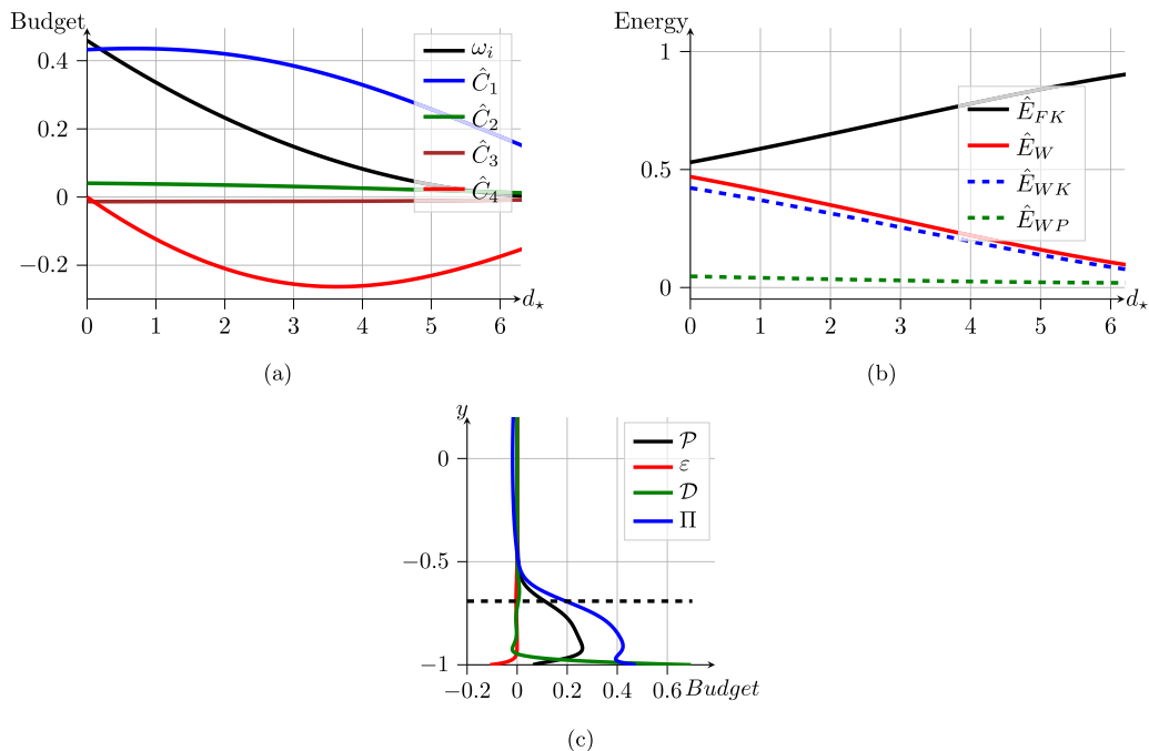
FIG. 23. Energy of most unstable varicose TWF mode as d_* is increased at \text{Re} = 10000 , B_* = 1 , and V_R = 3 . (a) Evolution of integrated total energy budget. (b) Distribution of total energy as fluid and wall contributions. (c) Cross-channel profile of the fluid kinetic energy budget for d_* = 4 . The wall-normal position of the critical layer is shown as a dashed-line.
