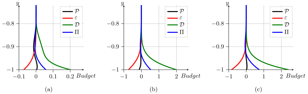
FIG. 21. Fluid kinetic energy budget profiles for most unstable divergence mode at Re = 10000 , B_* = 1 , and V_R = 2 and (a) d_* = 5 sinuous mode, (b) d_* = 5 varicose mode, and (c) d_* = 9 varicose mode.
