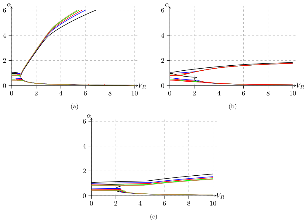
FIG. 10. Marginal curves for onset of sinuous instability at B_\star = 4 for \text{Re} = 10000, 40000, 80000, 160000, and 240000 (in black, blue, red, green, and brown respectively) and (a) d_\star = 0 , (b) d_\star = 10 , and (c) d_\star = 100 .
