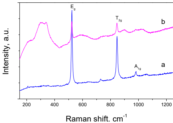
Fig. 3. Raman spectra of \gamma\text{-Si}_3\text{N}_4 before (a) and after (b) irradiation with \text{He}^+ ions.
