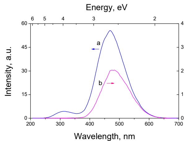
Fig. 4. CL spectra of \gamma\text{-Si}_3\text{N}_4 at T=5 K before (a) and after (b) irradiation with \text{He}^+ ions.
