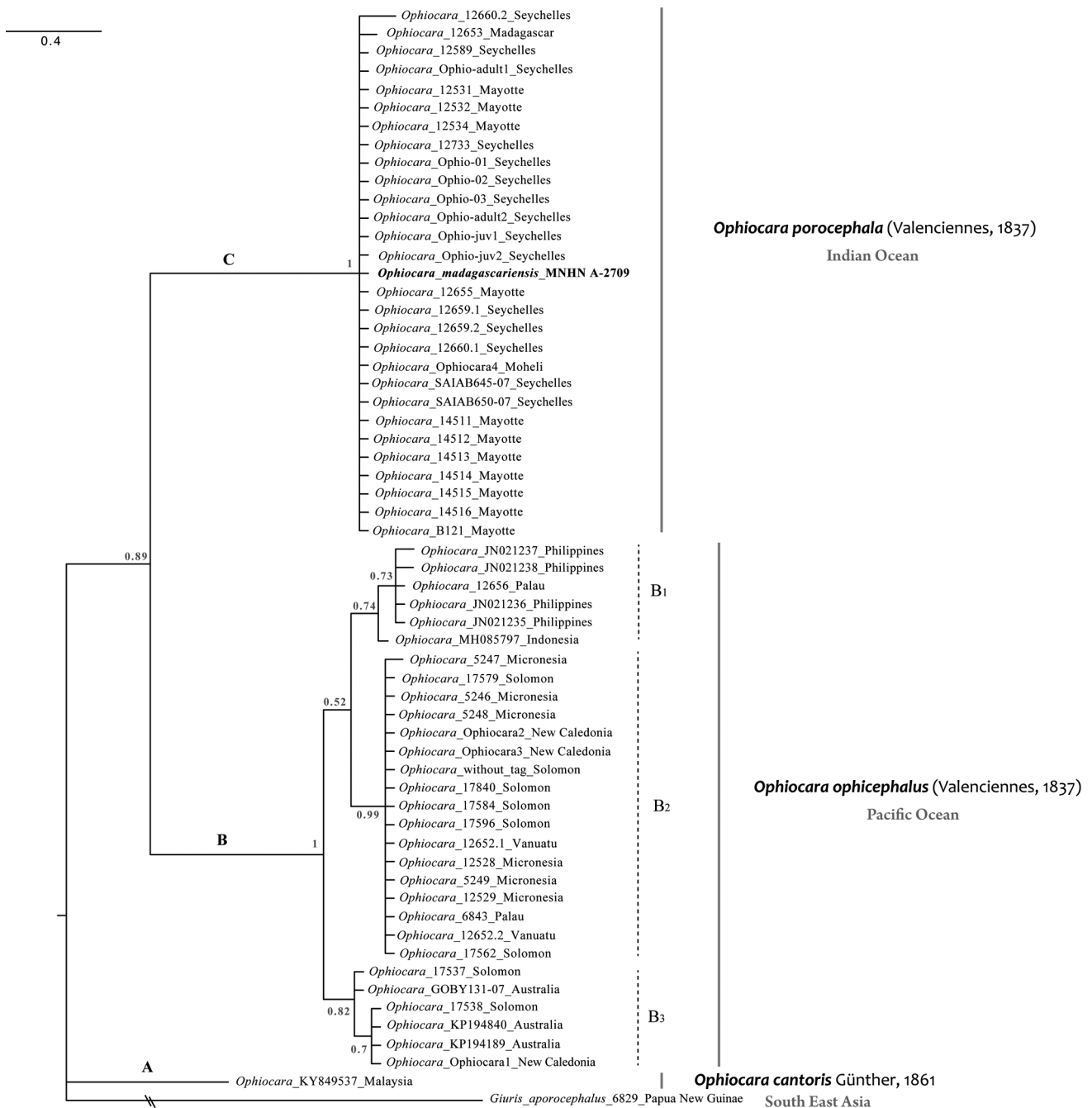
Figure 2. – Bayesian tree of the cytochrome c oxidase subunit ( COI ; 446 bp) for sequenced specimens of Ophiocara . Numbers at each node represent posterior probabilities.
