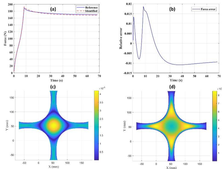
Figure 2: comparison of the obtained results with the reference data: (a) global force, (b) relative error of the global force, (c) relative error of the first in-plane principle stretch and (d) relative error of the second in-plane principle stretch
