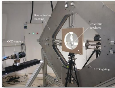
Figure 1: experimental set-up
