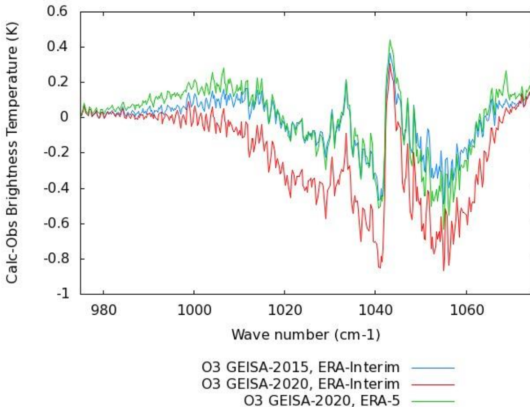
Figure 11: Comparison of ‘calculated-observed’ IASI residuals in the 975-1075 cm -1 spectral range and for tropical atmospheres, obtained using GEISA-2015 and GEISA-2020 O 3 line parameters and with different sources of ozone profiles used in the SPARTE chain: GEISA-2015 and ERA in blue, GEISA-2020 and ERA Interim in red and GEISA-2020 and ERA-5 in green).
