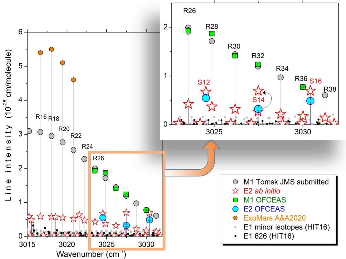
Fig. 5. Overview comparison of the different \text{CO}_2 transitions contributing to the absorption spectrum in the 3015-3032 \text{cm}^{-1} interval:
