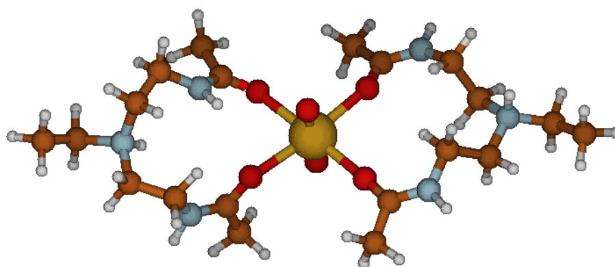
[UO_2^{2+}][LH^+]_2 complex
