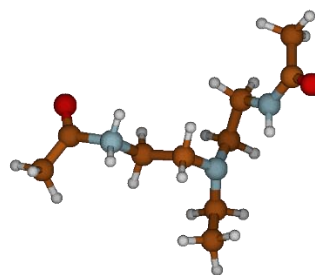
LH (protonated amide)
