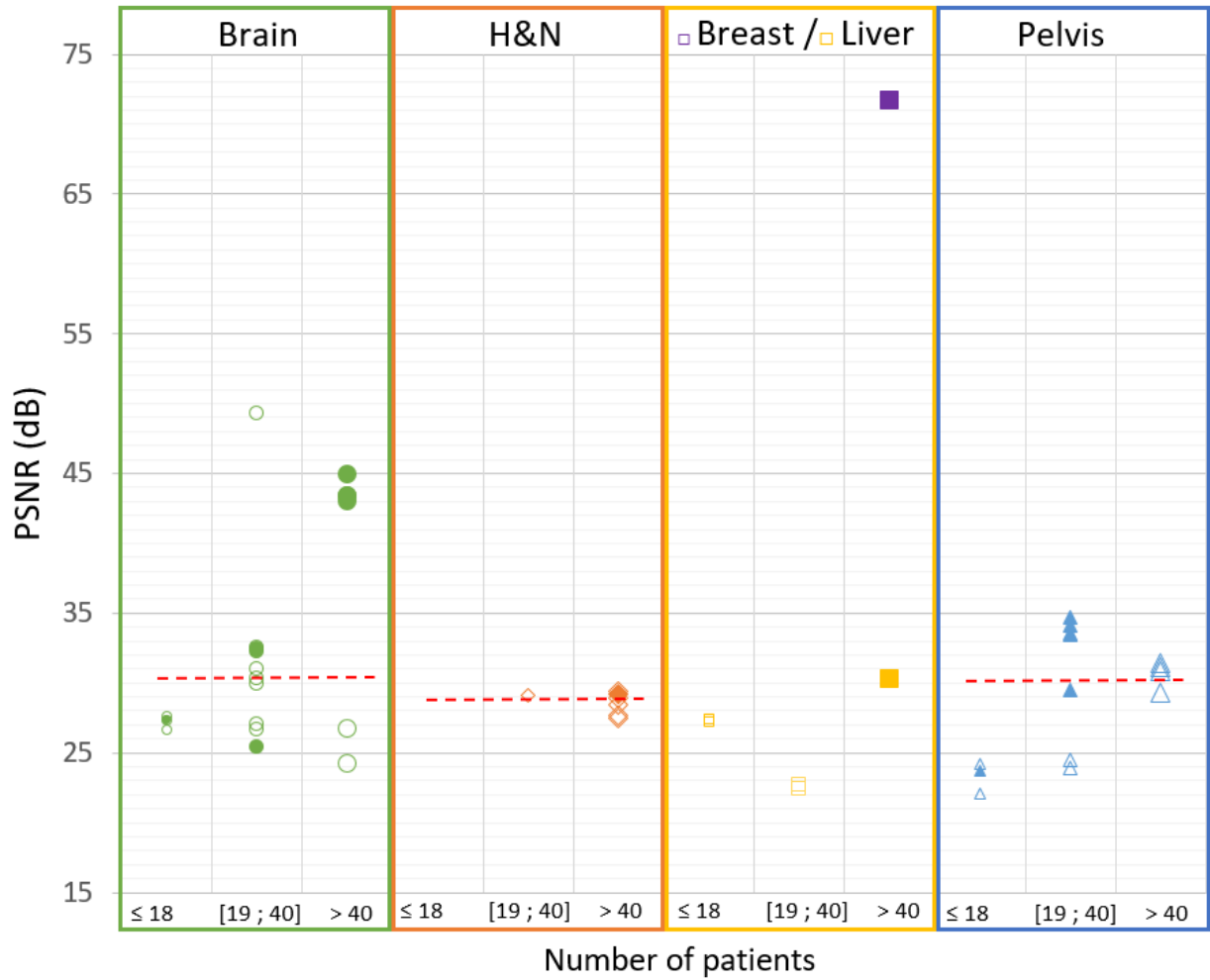
1 2 Figure 8: Peak signal-to-noise ratio (PSNR) results between reference CT and sCT generated with 3 deep learning methods in studies on the brain, head and neck, breast, liver, and pelvis 4 Full markers represent generator-only models and empty markers generative models with adversarial. 5 Results are divided into three categories: studies including less than 18 patients, studies including 19 to 6 40 patients and studies including more than 40 patients. 7 Red dotted lines represent the median values. The median values are: 30.3 dB for the brain, 28.9 dB for 8 H&N, and 30.2 dB for the pelvis. 9 The selected values are listed in the Additional tables 1 to 4.
