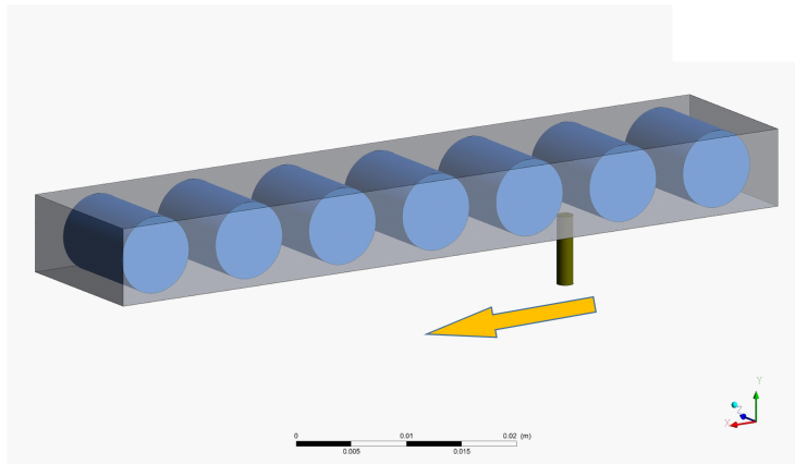
Figure 6: Simulation model for roller rotating validation
