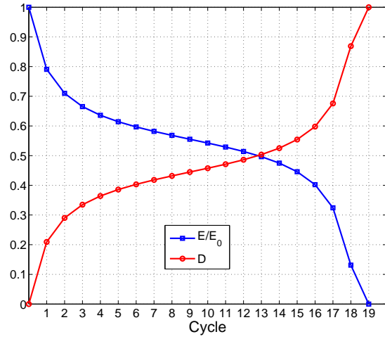
Figure 11: Evolution of damage and Young modulus with cycles for \mu = 0.5
