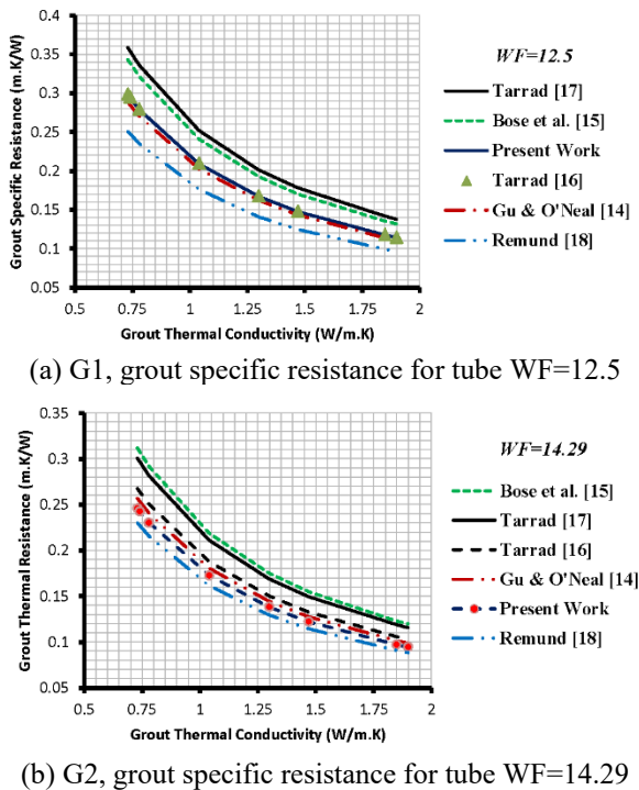
Figure 3. Comparison of grout specific thermal resistance at ( S_p/d_o ) of 3.3
