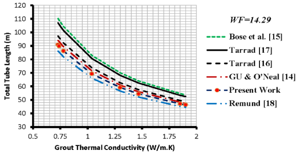
(b) G2, total U-tube length for \Delta T_m = 15^\circ\text{C}
