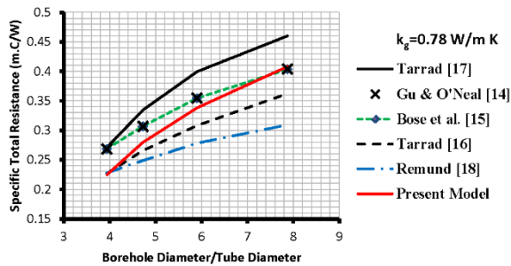
(b) Total thermal resistance variation
