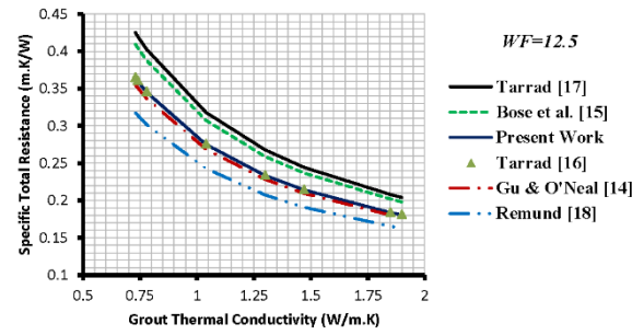
(a) G1, specific total thermal resistance at tube WF=12.5
