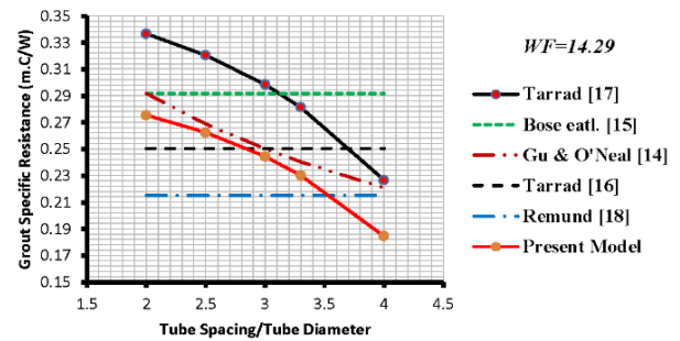
Figure 6. Variation of grout thermal resistance with U-tube legs spacing at fixed D_B/d_o
