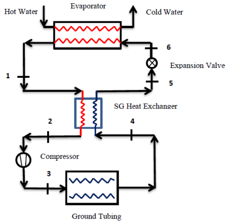
(a) A schematic diagram of the hypothetical heat pump system
