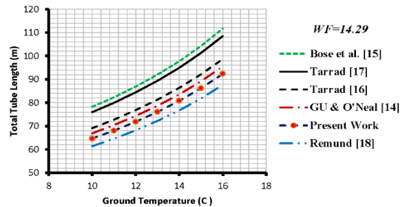
Figure 8. Comparison of U-tube length at k_g of 0.78 W/m.K
