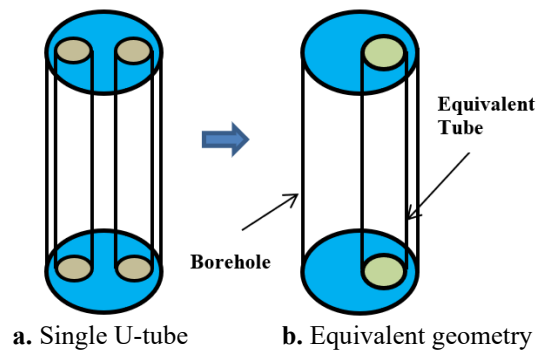
Figure 1. A schematic presentation of the present model
