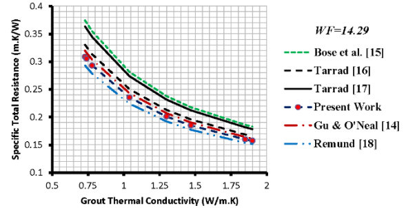
(b) G2, specific total thermal resistance tube WF=14.29
