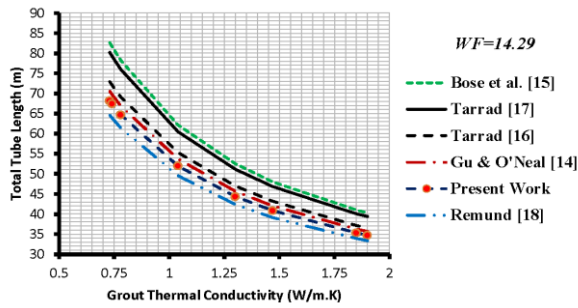
(a) G2, total U-tube length for \Delta T_m = 20^\circ\text{C}
