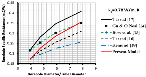
(a) Borehole thermal resistance variation
