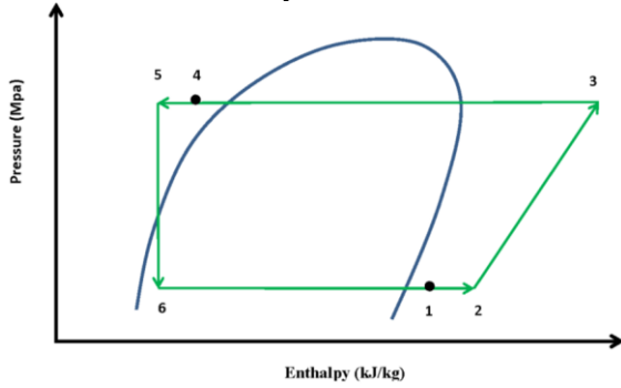
(b) A (p-h) diagram of the hypothetical geothermal heat pump system [22]
