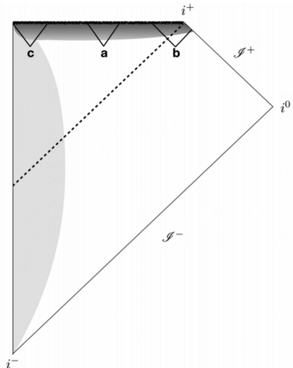
FIG. 1. The Carter-Penrose diagram of a Schwarzschild black hole until the onset of quantum gravity. The light gray region is the collapsing star. The dark gray region is where quantum gravity becomes relevant.
