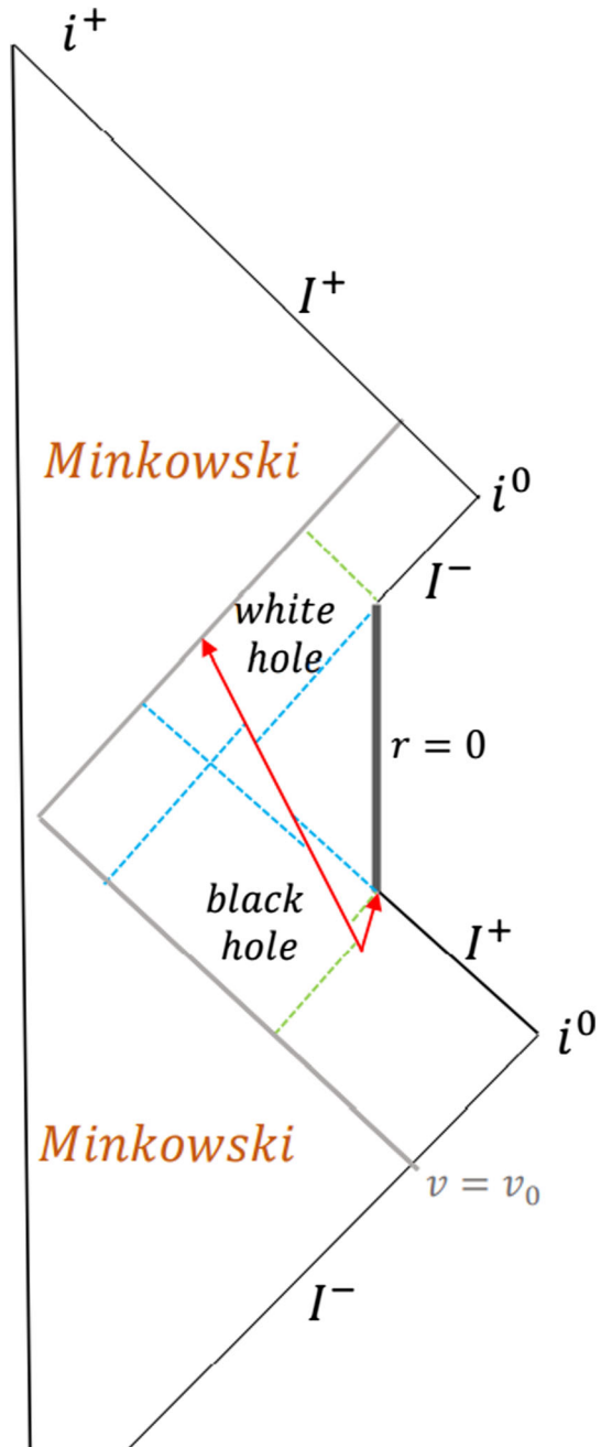
FIG. 13. Massive Hawking radiation quanta enter the quantum region and make the inner (and outer) horizon shrink. (Depicted without the gluing of the two asymptotic regions).
