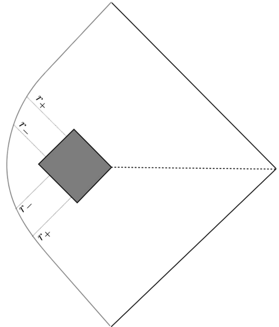
FIG. 6. The spacetime of the black to white charged transition outside the star.
