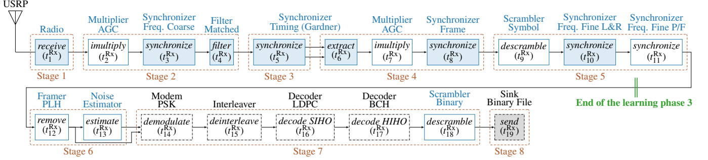
Fig. 3. DVB-S2 software receiver: acquisition phase 3 & transmission phase.
