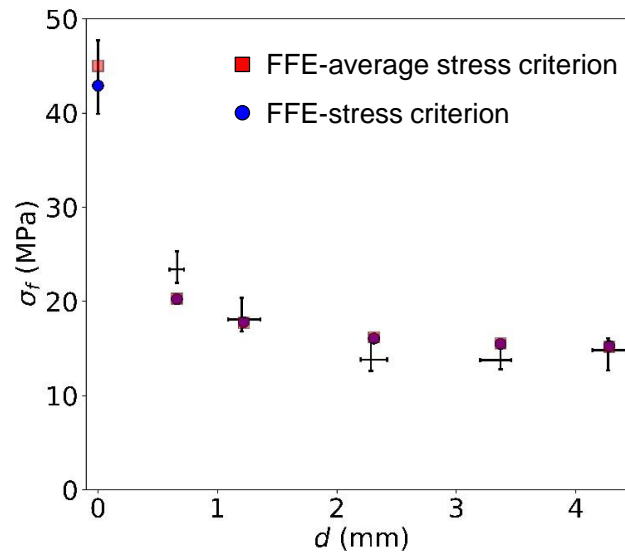
Fig. 10: Failure stress predicted by the CC employing the stress criterion (blue dots, \sigma_c = 42.9 \text{ MPa} , G_c = 92 \text{ J/m}^2 ) or its average version (red squares, \sigma_c = 45 \text{ MPa} , G_c = 140 \text{ J/m}^2 ) as a function of the circular hole diameter.
