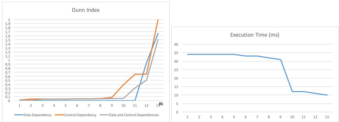
(a) Dunn Index of the clustering results
