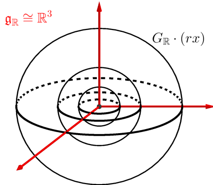
FIGURE 1. Adjoint orbits for SU(2) .
