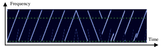
Fig 3: Example of observed LoRa transmitted frame during the labwork
