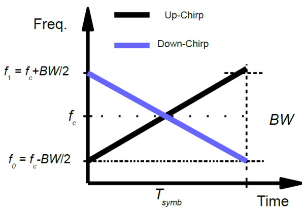
Fig 2: Spectrogram of the up chirp and down chirp from [3]
