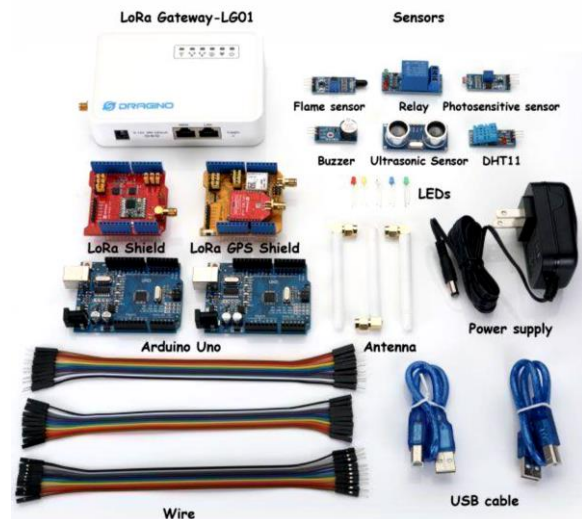
Fig 4: LoRa IoT development kit from Dragino [5]
