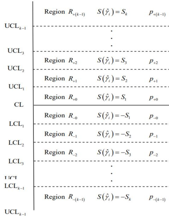
Fig 1. k regions above and below the center line of the RS- \gamma chart (Teoh et al., 2016)
