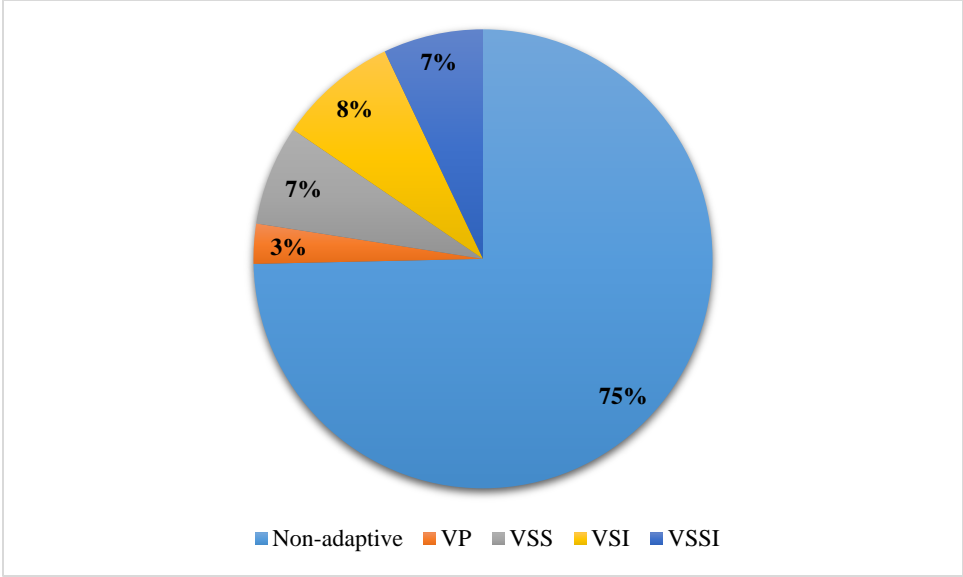
Fig 7. Percentage of papers based on the types of adaptive control charts
