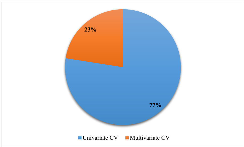
Fig 4. Percentage of papers based on the types of quality characteristics
