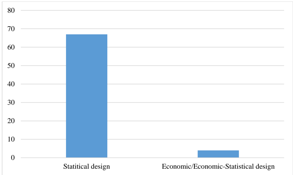
Fig 3. Percentage of published papers in different areas of SPM
