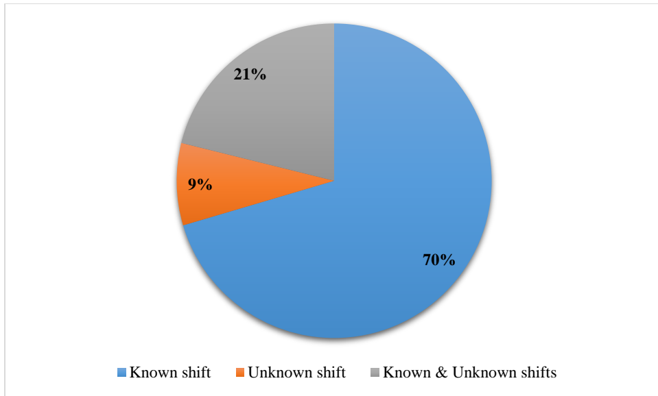
Fig 5. Percentage of papers based on the types of shift sizes
