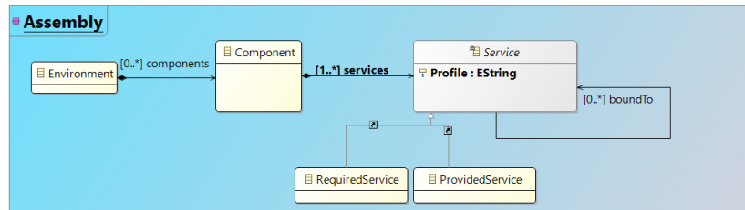
Figure 4: Assembly metamodel
