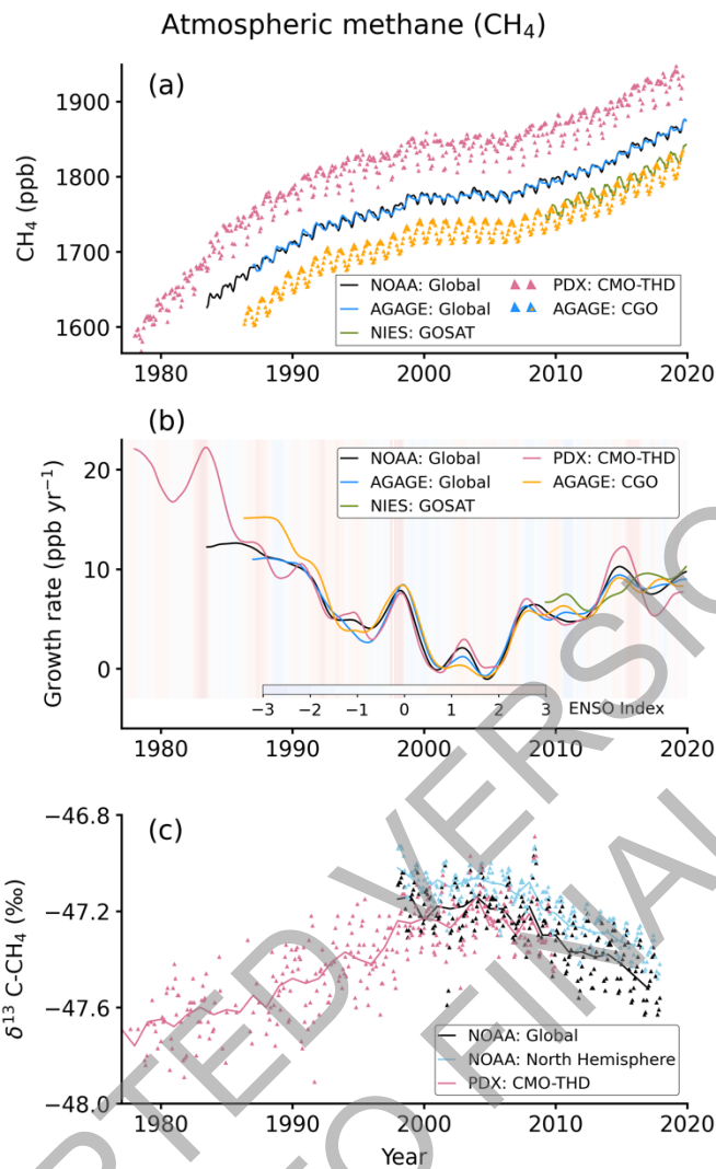
Figure 5.13: Time series of CH 4 concentrations, growth rates and isotopic composition. a) CH 4 concentrations, b) CH 4 growth rates, c) \delta^{13}\text{-CH}_4 . Data from selected site networks operated by NOAA (Dlugokencky et al., 2003), AGAGE (Prinn et al., 2018) and PDX (Portland State University) (Rice et al., 2016). To maintain clarity, data from many other measurement networks are not included here, and all measurements are shown in WMO X2004ACH 4 global calibration standard. Global mean values of XCH 4 (total-column), retrieved from radiation spectra measured by the greenhouse gases observation satellite (GOSAT) are shown in panels (a) and (b). Cape Grim Observatory (CGO; 41°S, 145°E) and Trinidad Head (THD; 41°N, 124°W) data are taken from the AGAGE network, NOAA global and northern hemispheric (NH) means for \delta^{13}\text{C} are calculated from 10 and 6 sites, respectively. The PDX data adjusted to NH (period: 1977–2000) are merged with THD (period: 2001–2019) for CH 4 concentration and growth rate analysis, and PDX and NOAA NH means of \delta^{13}\text{C} data are used for joint interpretation of long-term trends analysis. The multivariate ENSO index (MEI) is shown in panel (b). Further details on data sources and processing are available in the chapter data table (Table 5.SM.6).
