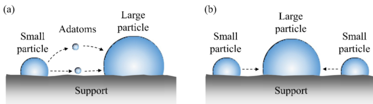
Figure 7. Conceptual models representing main mechanisms of metal particles sintering (via adatoms migration (a) or small particles agglomeration (b)) due to thermal degradation. Ochoa et al. [17].
