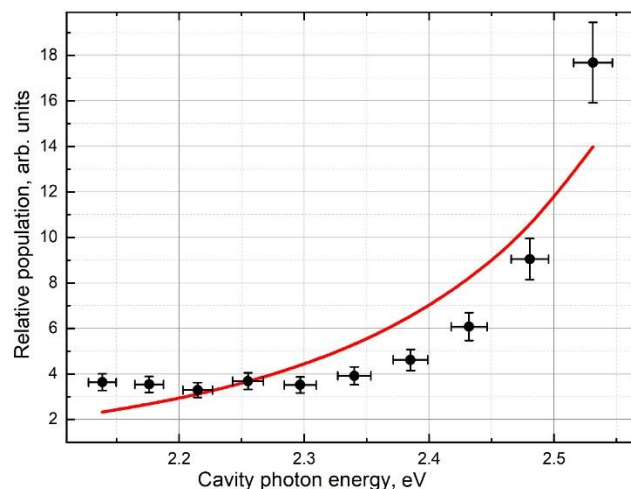
Figure 6. Experimentally observed data (black dots) and theoretically modelled results (red line) for dependences of the relative population of the lower polaritonic branch on the cavity detuning. The relative population is the emission intensity from the lower polariton divided by the corresponding Hopfield coefficient determining the fraction of the cavity photon.
