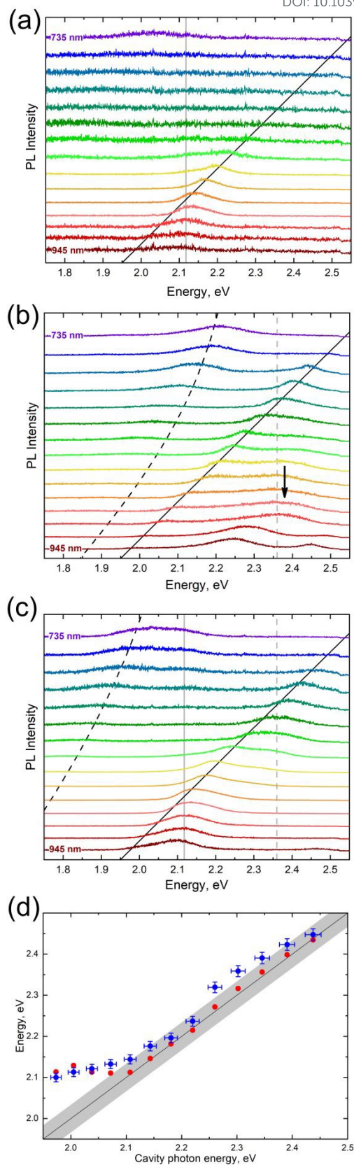
Figure 2. The PL properties of the hybrid system at different cavity mode detunings. The PL spectra recorded at distances between the mirrors varied from 735 to 945 nm at a 15-nm step (from top to bottom in panels a-c) for microcavity filled with the molecular beacons labelled with TAMRA (a), FAM (b), or the
