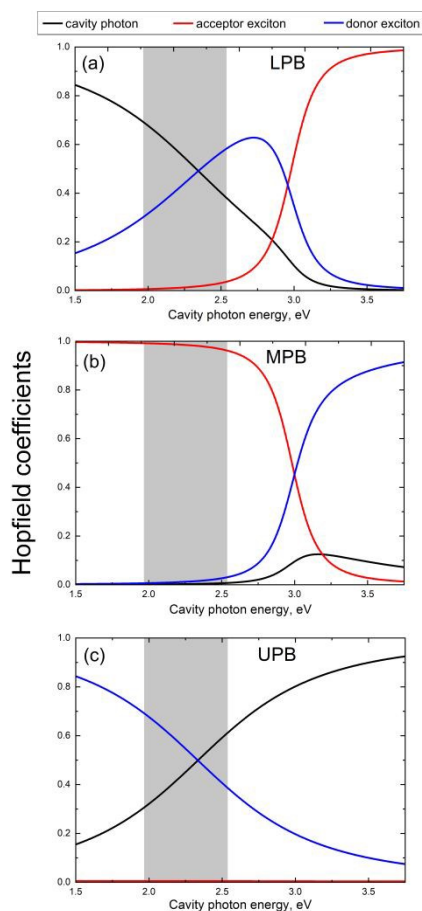
Figure 5. The Hopfield coefficients of the lower (a), middle (b), and upper (c) polaritonic branches calculated using the Jaynes–Cummings model for the microcavity filled with molecular beacons labelled with both FAM and TAMRA dyes. The grey area shows the range of the cavity mode detuning measured experimentally.
