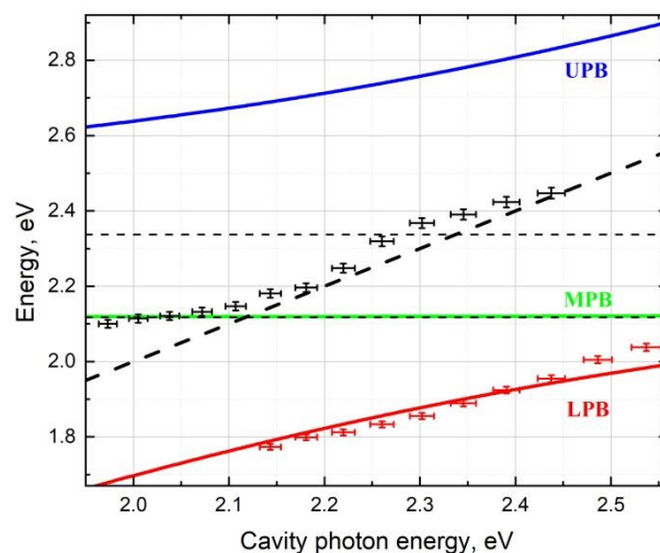
Figure 4. The energies of the lower (red), middle (green), and upper (dark blue) polariton branches at different cavity detunings experimentally derived from the PL spectra (dots) and theoretically calculated (solid lines). The black dots correspond to the emission from weakly coupled dye molecules. The horizontal and inclined black dashed lines show the energies of the donor and acceptor exciton transitions and the cavity mode energy, respectively.
