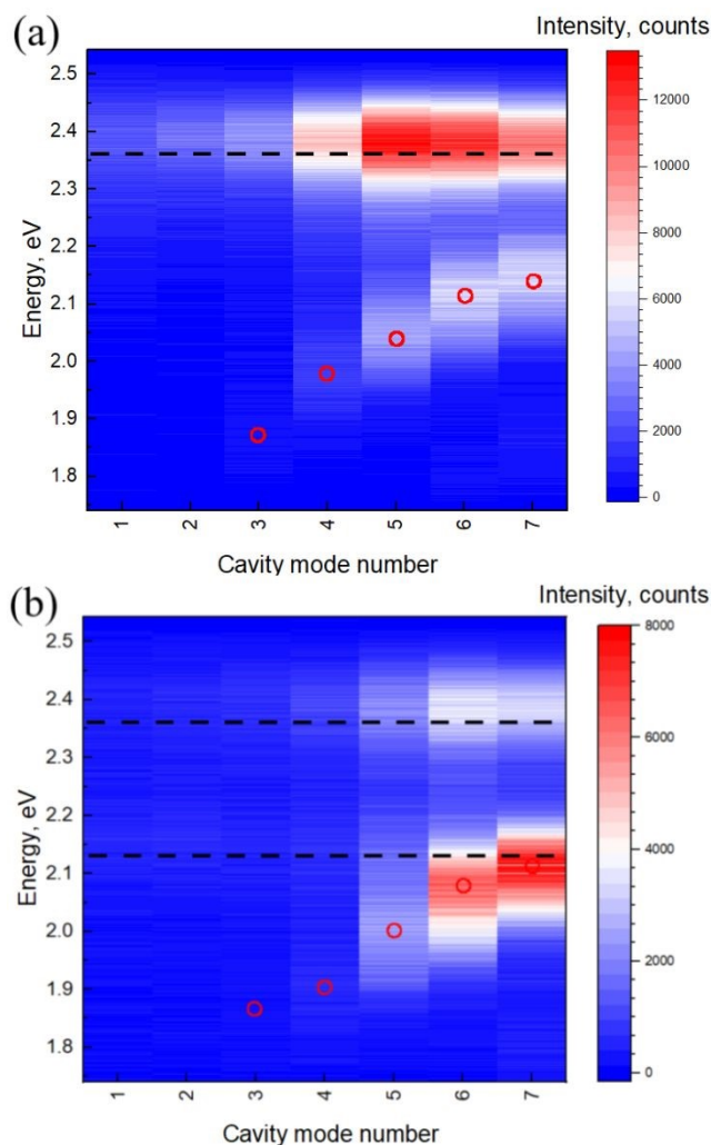
Figure 3. PL at zero detuning (the cavity photon energy corresponds to the energy of the donor emission maximum) for distances between the cavity mirrors varying from 199 to 1393 nm at a step of \lambda/2 for a microcavity filled with the molecular beacons labelled with FAM (a), or the FAM–TAMRA donor–acceptor pair operating in the FRET regime (b). Black dashed lines show the energies of the donor (2.36 eV) and acceptor (2.13 eV) emission maxima, red circles mark the spectral positions of the emission peaks corresponding to the lower polariton.
