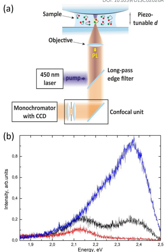
Figure 1. (a) The schematic of the tuneable microcavity. (b) The PL emission spectra of the solutions containing molecular beacons labelled with FAM alone (blue), TAMRA alone (red), and both FAM and TAMRA (black) dyes. All samples were located outside the microcavity. The PL spectra were excited at 450 nm. The concentrations of the dye molecules in the sample solutions were about 100 \mu\text{M} in all experiments. The molecular beacons are drawn not to scale.
