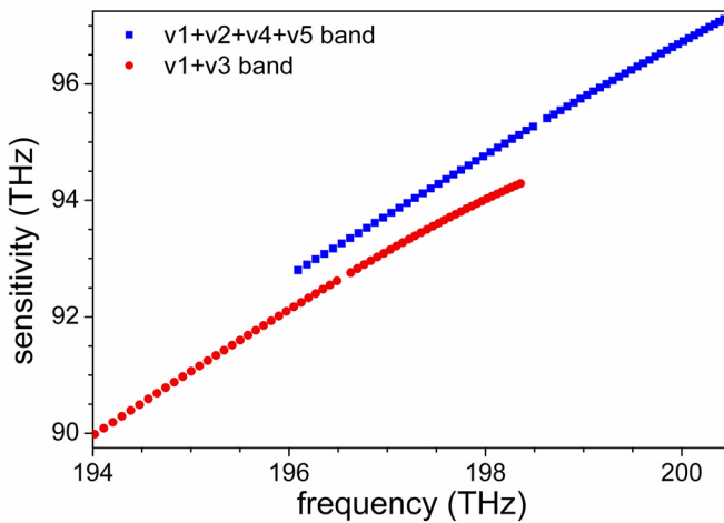
Fig. 3 Dependence of the sensitivity of the v_1 + v_3 and v_1 + v_2 + v_4 + v_5 band transitions on the calculated rovibrational frequency.
