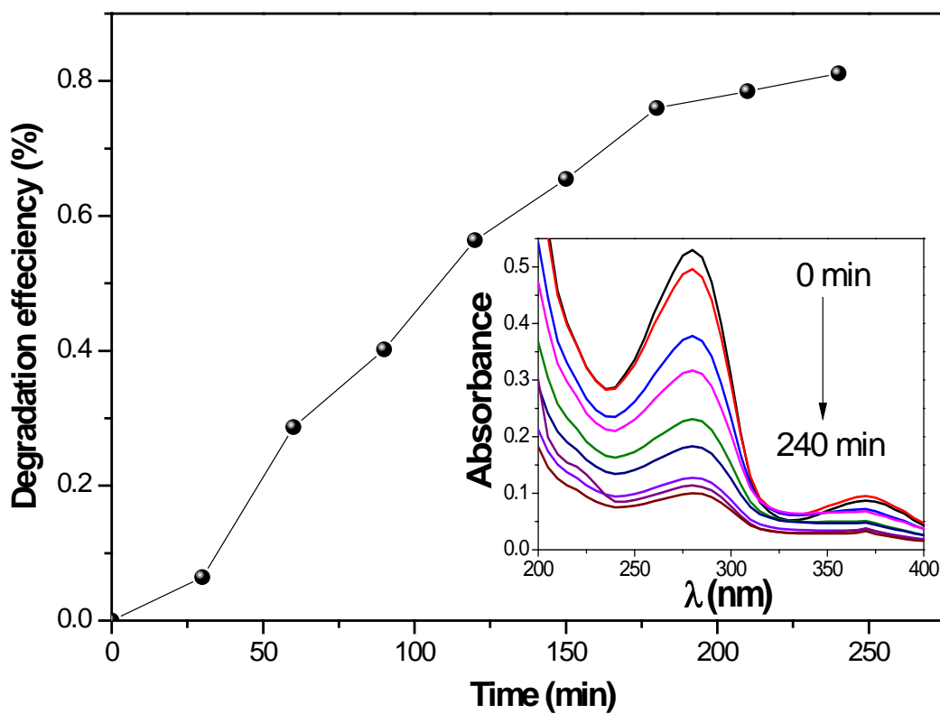
Fig. 6 Photocatalytic activity of Bi 12 ZnO 20 for Cefuroxime degradation. Inset: Associated UV-vis spectra.
