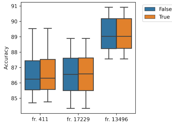
Figure 13: Accuracy per manuscript given the status (colored or original grayversion of microfilms).
