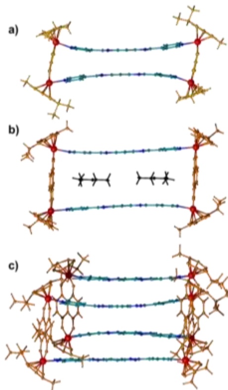
Figure 3. Single crystal X-ray diffraction structures of a) Oxa 2 BBI 2 , b) Naph 2 BBI 2 (including two solvent molecules, Et 2 O) and c) MM+ simulation of ( Naph 2 BBI 2 ) 2 . For a) and b) anions are omitted for clarity.
