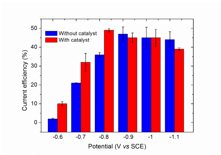
Fig. 7. Current efficiency of iohexol deiodination with and without catalyst after 1 h electroreduction for potentials ranging from -0.6 V to -1.1 V vs SCE. ( 0.5 mmol L -1 iohexol in a 0.5 mol L -1 pH=7 phosphate buffer solution with 100 \mu mol L -1 vitamin B12). Error bars are based on duplicate experiments.
