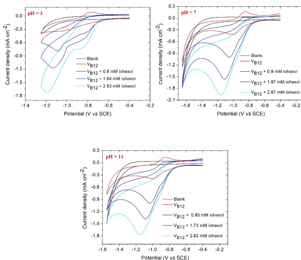
Fig. 3. Cyclic voltammograms of 2 mmol L -1 vitamin B12 (V B12 ) in 0.1 mol L -1 Na 2 SO 4 + different concentrations of iohexol at pH 3, 7, 11 (first scan). Blank: cyclic voltammetry in 0.1 mol L -1 Na 2 SO 4 . Scan rate: 20 mV s -1 .
