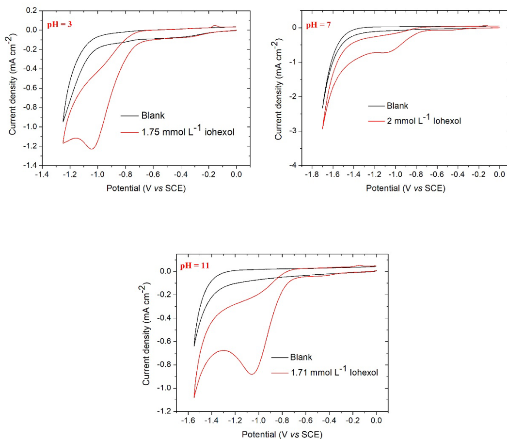
Fig. 2. Cyclic voltammograms in 0.1 mol L -1 Na 2 SO 4 without (—) (blank) and with (—) iohexol at pH 3, 7, 11. Scan rate: 20 mV s -1 .
