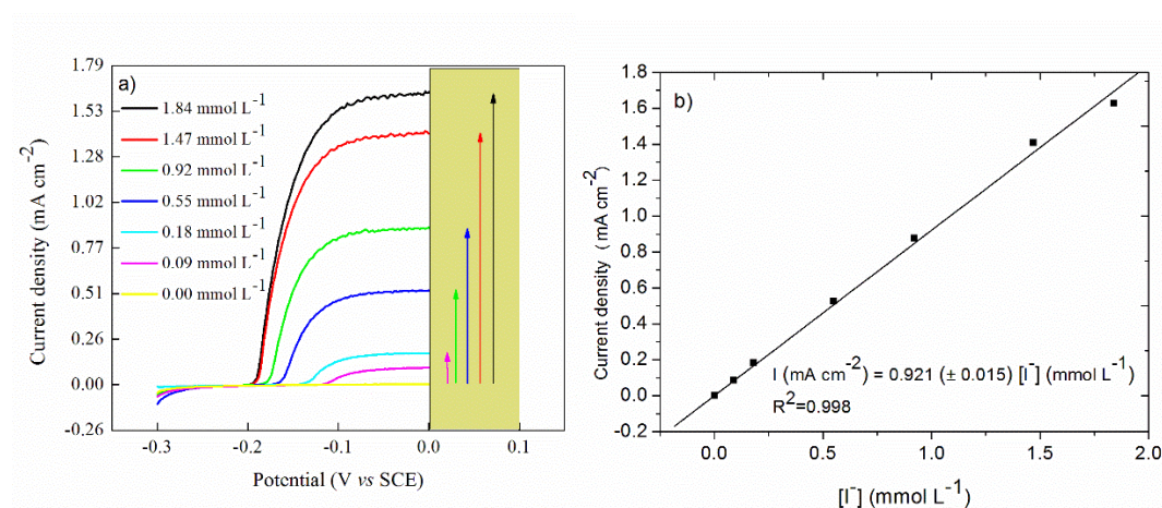
Fig. 1. a) Linear sweep voltammogram at a silver rotating disc electrode ( 0.20 \text{ cm}^2 ) of different concentrations of KI, scan rate: 20 \text{ mV s}^{-1} , rotating speed: 1000 rpm. Potential range: - 300 – 100 mV b) Calibration curve
