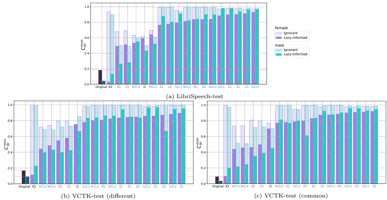
Figure 2: C_{llr}^{\min} results on the test datasets for different anonymization systems and for original data; oa : original enrollment and anonymized trial data; aa : both enrolment and trial data are anonymized. Blue and red colors in the system notations indicate systems developed from B1 and B2 respectively. The results are ordered by C_{llr}^{\min} values on female speakers for the lazy-informed attack model. Larger C_{llr}^{\min} values correspond to better privacy.
