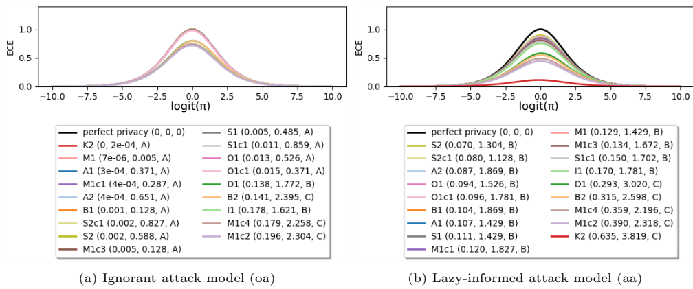
Figure 5: ZEBRA assessment with ECE profiles on VCTK-test (different) for female speakers.
