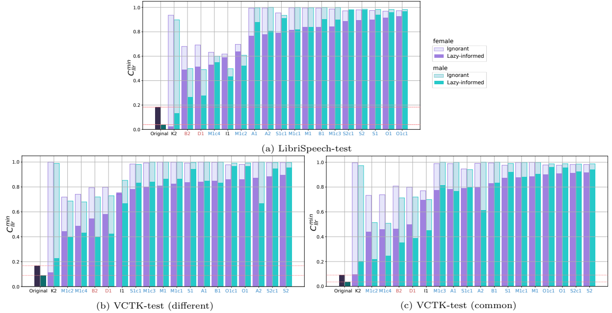
Figure 2: C_{llr}^{min} results on the test datasets for different anonymization systems and for original data; oa: original enrollment and anonymized trial data; and aa: both enrolment and trial data are anonymized. Blue and red colors in the system notations indicate systems developed from B1 and B2 respectively. The results are ordered by C_{llr}^{min} values on female speakers for the lazy-informed attack model. Larger C_{llr}^{min} values correspond to better privacy.
