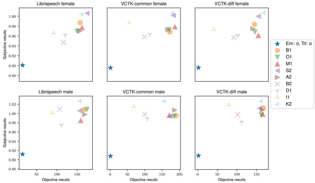
Figure 29: Objective versus subjective C_{1lr} .
