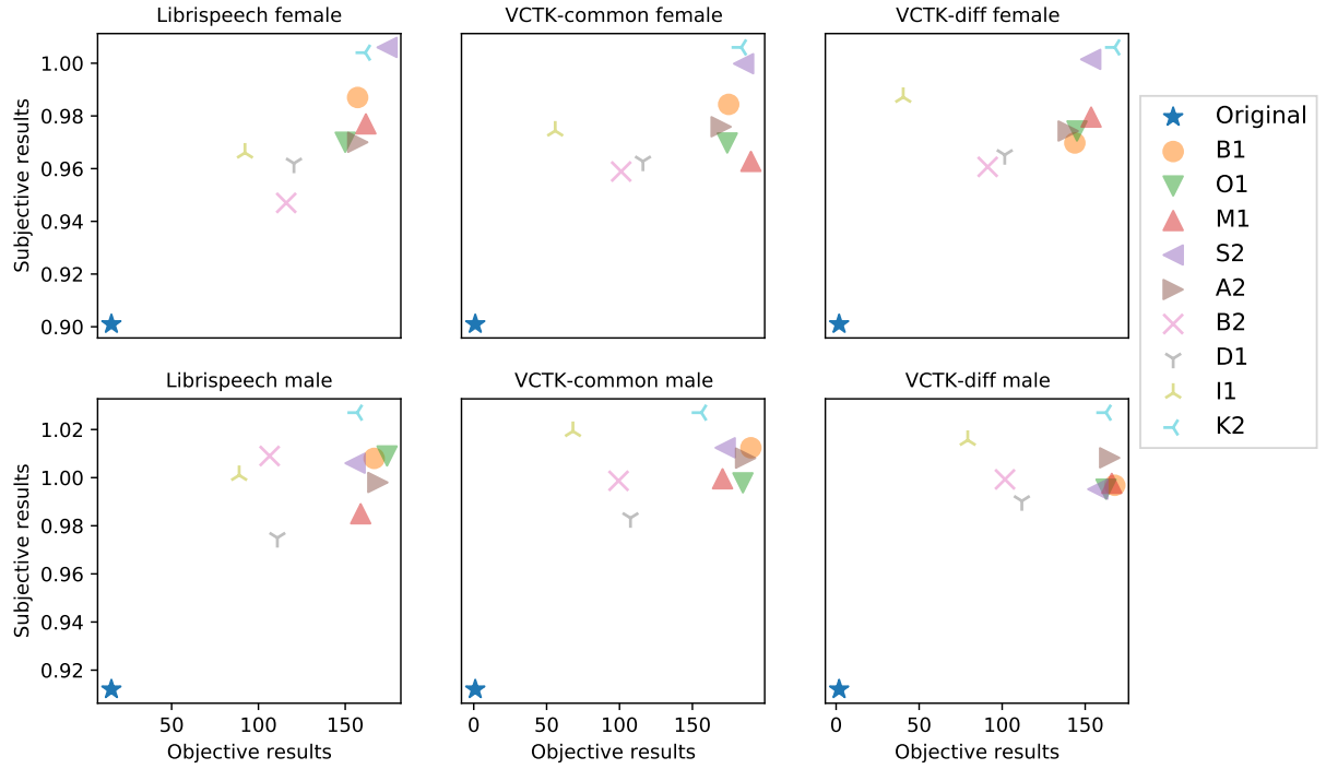
Figure 29: Objective (ignorant attack model) versus subjective C_{illr} .
