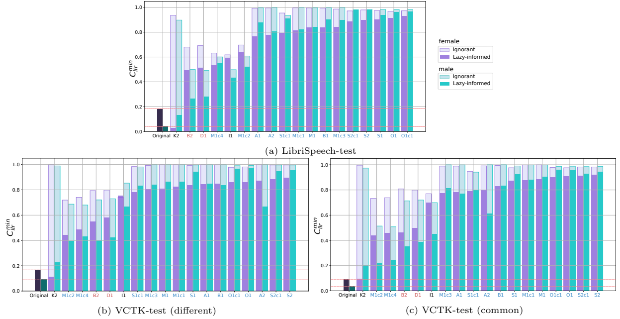
Figure 2: C_{llr}^{\min} results on the test datasets for different anonymization systems and for original data; oa : original enrollment and anonymized trial data; and aa : both enrolment and trial data are anonymized. Blue and red colors in the system notations indicate systems developed from B1 and B2 respectively. The results are ordered by C_{llr}^{\min} values on female speakers for the lazy-informed attack model. Larger C_{llr}^{\min} values correspond to better privacy.
