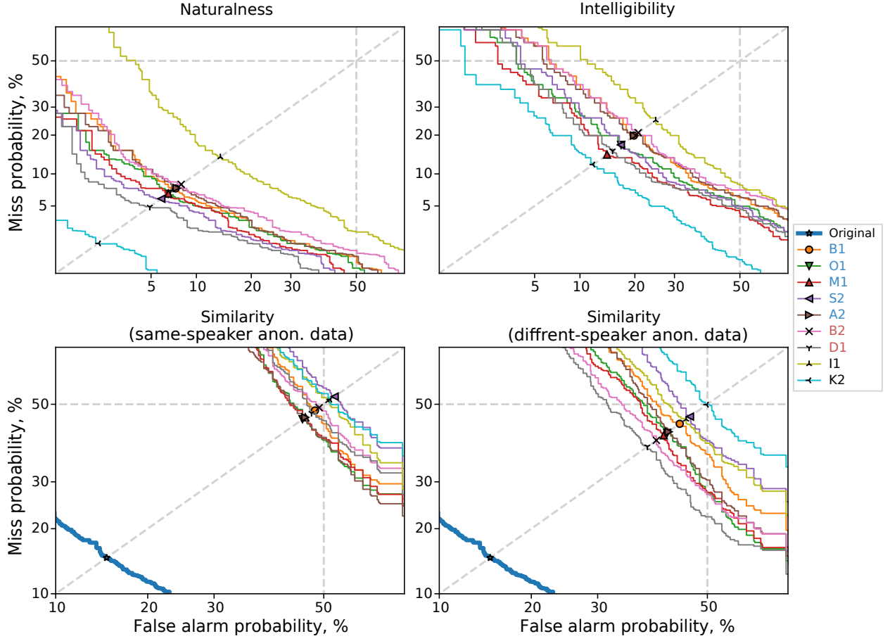
Figure 25: DET curves based on subjective evaluation scores pooled over LibriSpeech-test and VCTK-test datasets.
