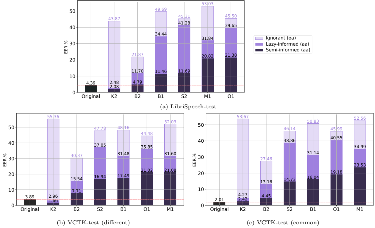
Figure 15: EER results achieved by different anonymization systems on the test datasets against the three attack models, compared to the EER achieved on the original data.
