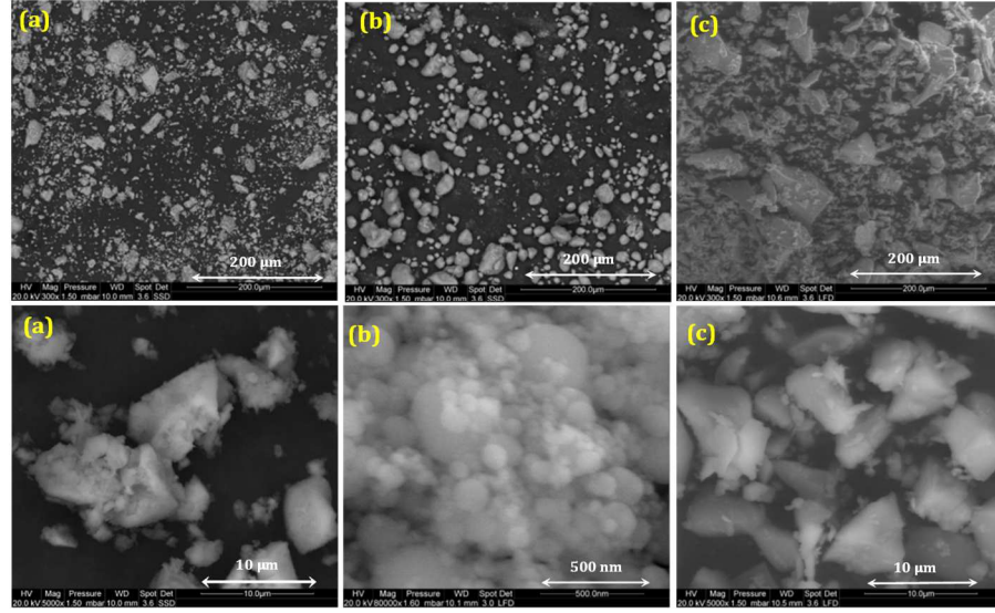
Fig. 3: SEM images of CEMI (a), silica fume (b) and glass powder (c).
