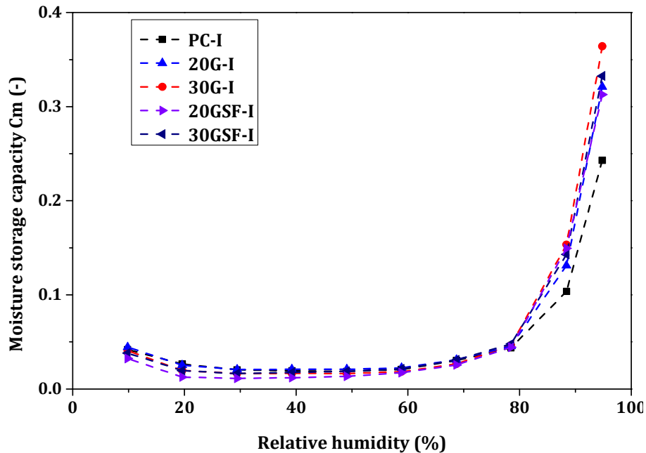
Fig. 17: Moisture storage capacity of the concretes studied.
