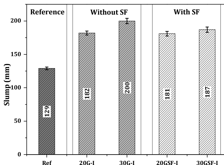
Fig. 5: Workability of the studied concretes.
