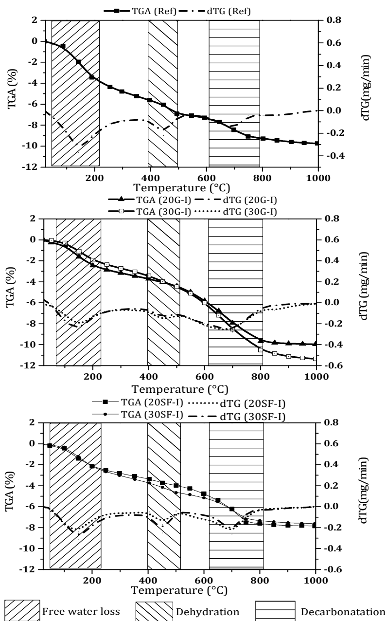
Fig. 11: TG and dTG curves of the studied concretes (solid line: TG; dash line: dTG).
