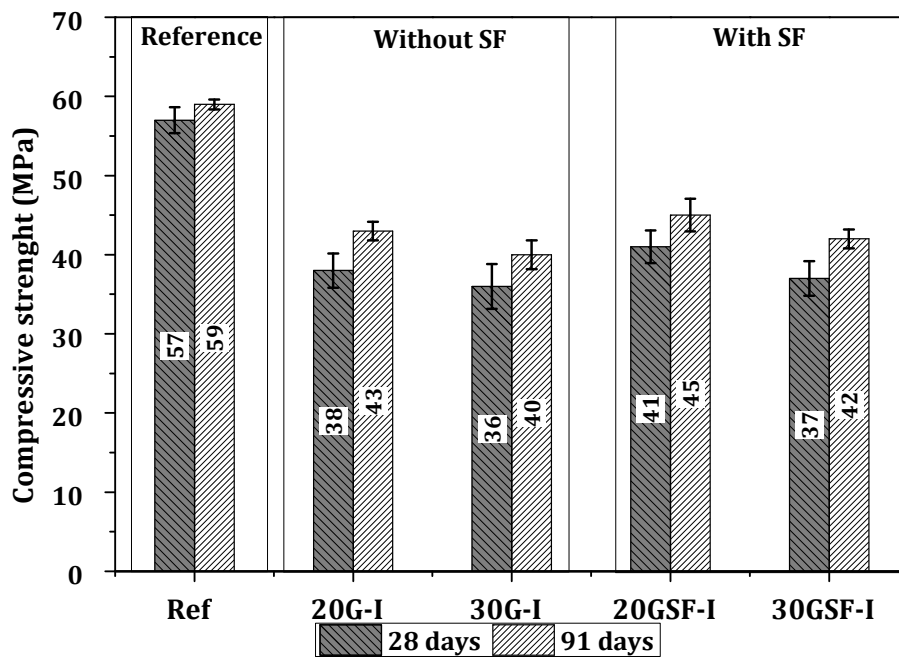
Fig. 8: Compressive strength of the concretes used.
