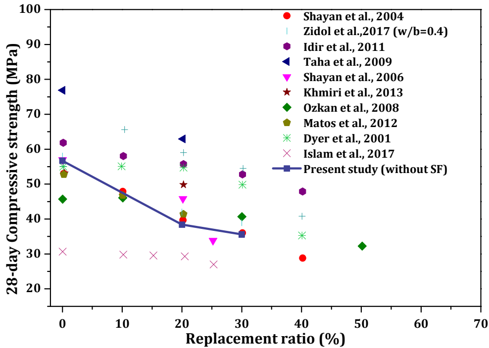
Fig.9: Effect of GP replacement ratio on the 28day compressive strength of mortar and concrete.
