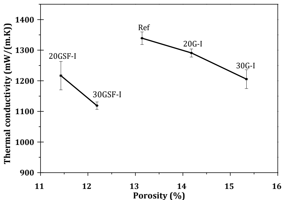
Fig.14: Thermal conductivity of studied concrete.
