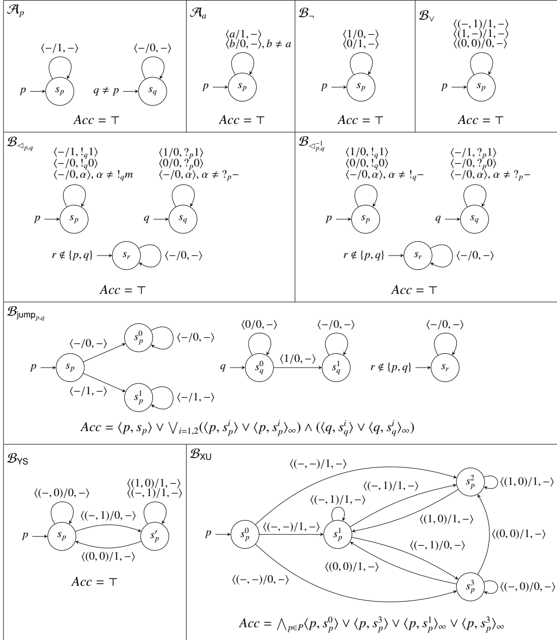
Figure 9: Transducers used to define \mathcal{A}_c . In a transition labeled \langle a/b, \alpha \rangle , a is the input letter, b is the output letter, and \alpha is either empty or a read or write action. Notice that in \mathcal{B}_{\triangleleft_{p,q}} , the automaton for process q has no transitions reading \langle c/0, ?_p d \rangle , with c \neq d , hence a wrong guess by process p cannot lead to an accepting run. The acceptance condition \top means true and is always satisfied.
