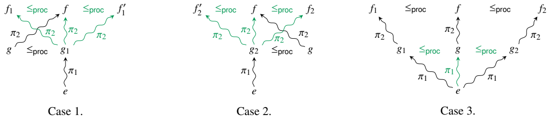
Figure 3: Proof of Lemma 4.
